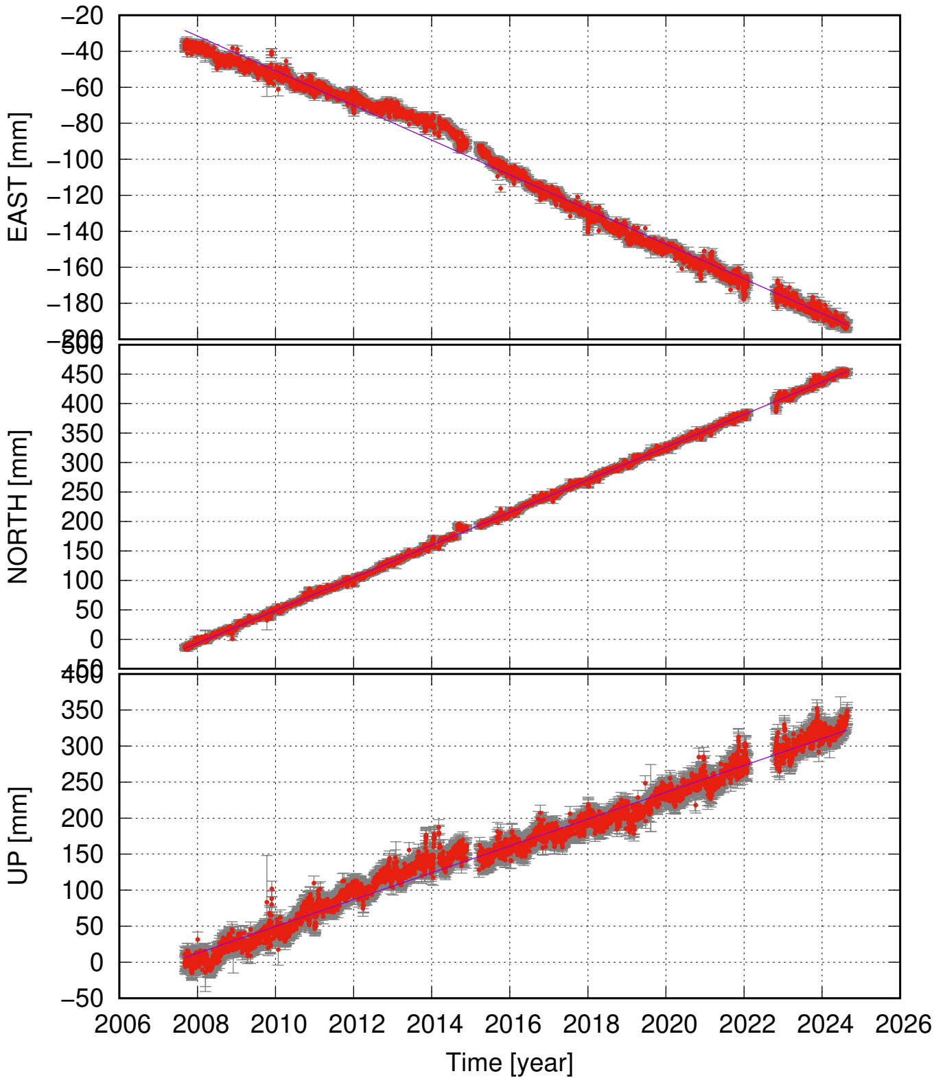
FJOC (64.87, -18.01) time series (ITRF 2014) v_e = -9.63 \pm 0.27 ; v_n = 27.70 \pm 0.18 ; v_u = 18.61 \pm 0.71 mm/yr
