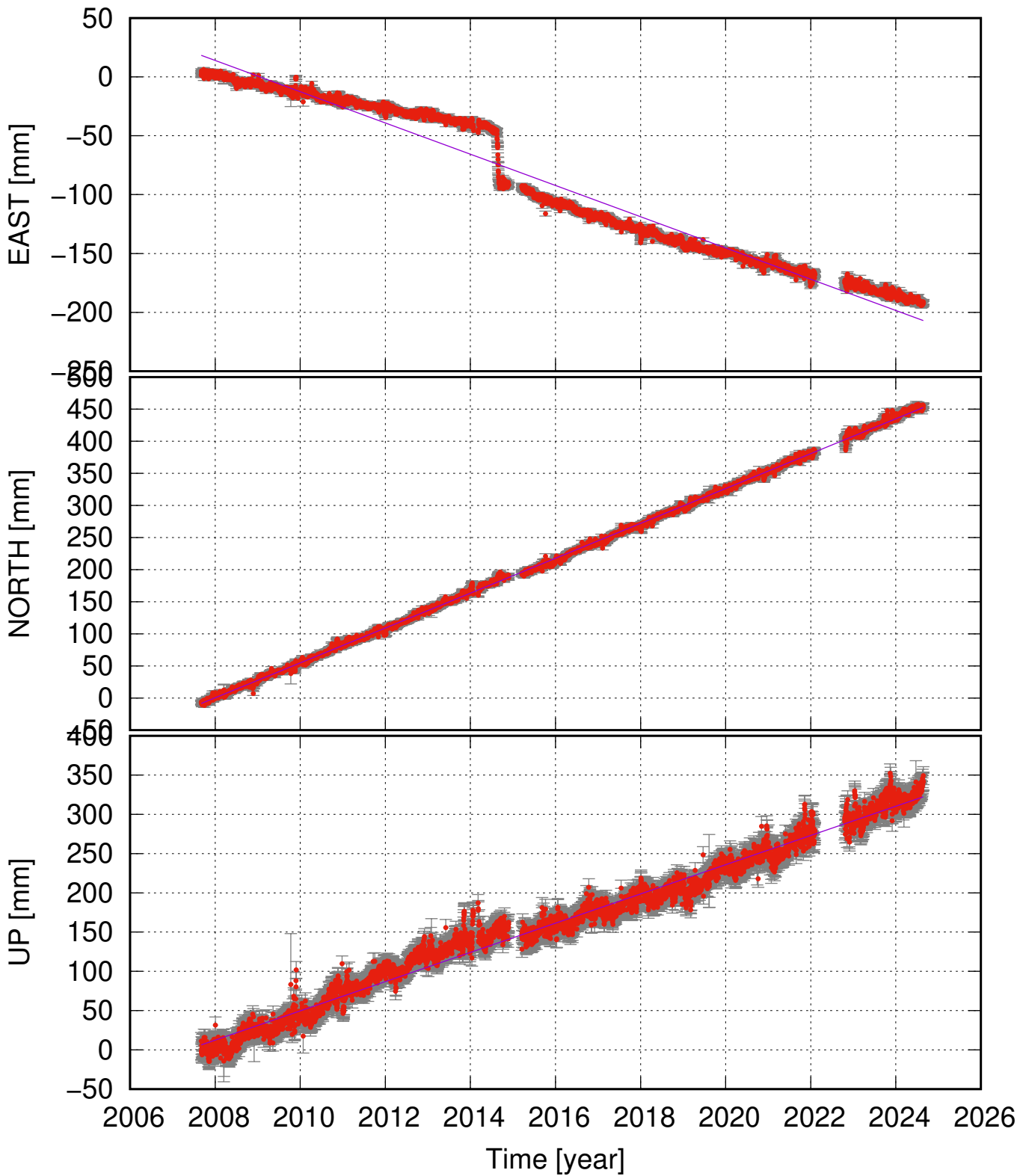
FJOC (64.87, -18.01) time series (ITRF 2014) v_e = -13.27 \pm 0.74 ; v_n = 27.16 \pm 0.19 ; v_u = 18.61 \pm 0.72 mm/yr
