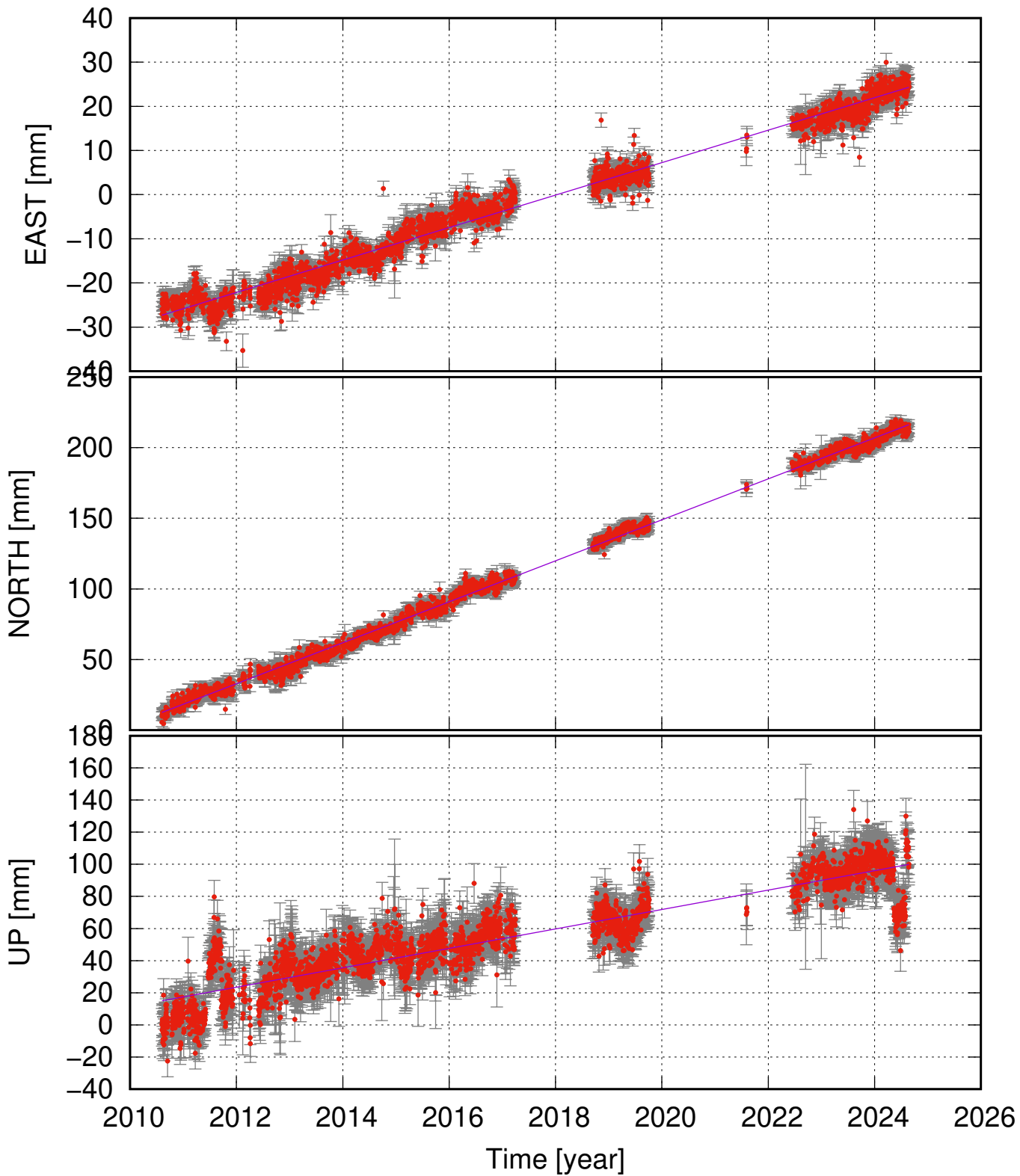
FIM2 (63.61, -19.43) time series (ITRF 2014) v_e = 3.68 \pm 0.16 ; v_n = 14.51 \pm 0.23 ; v_u = 6.05 \pm 0.81 mm/yr
