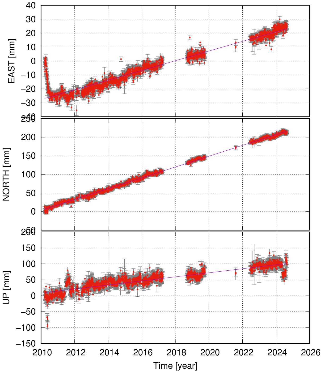
FIM2 (63.61, -19.43) time series (ITRF 2014) v_e = 3.47 \pm 0.28 ; v_n = 14.55 \pm 0.23 ; v_u = 6.35 \pm 0.85 mm/yr
