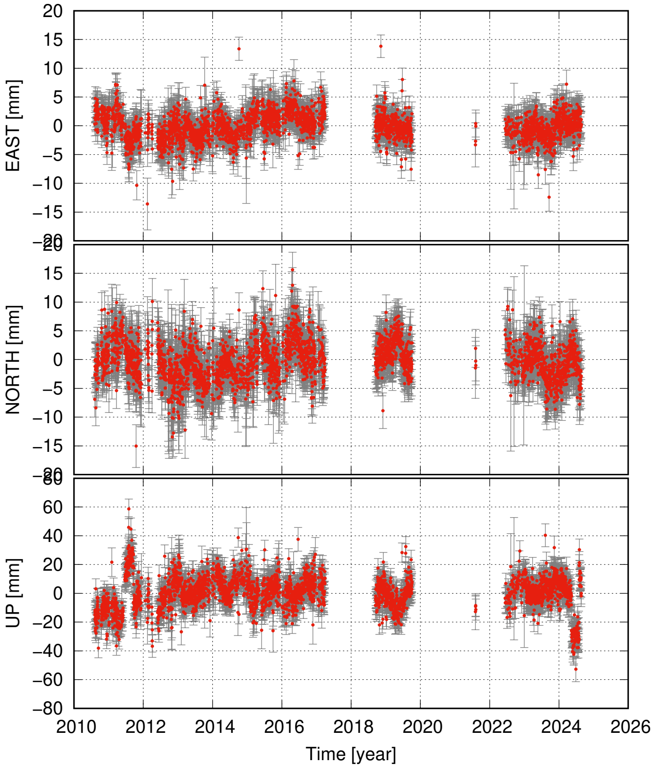
FIM2 residual time series (some major events removed as well)
