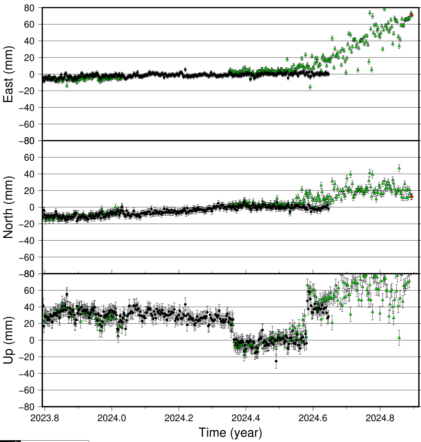
FIM2 time series (IGS 2014), last 400 days
