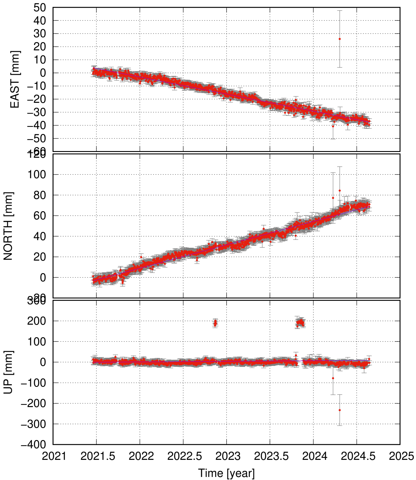
FIHO (64.69, -22.15) time series (ITRF 2014) v_e = -13.02 \pm 0.80 ; v_n = 22.69 \pm 0.91 ; v_u = 2.79 \pm 10.70 mm/yr
