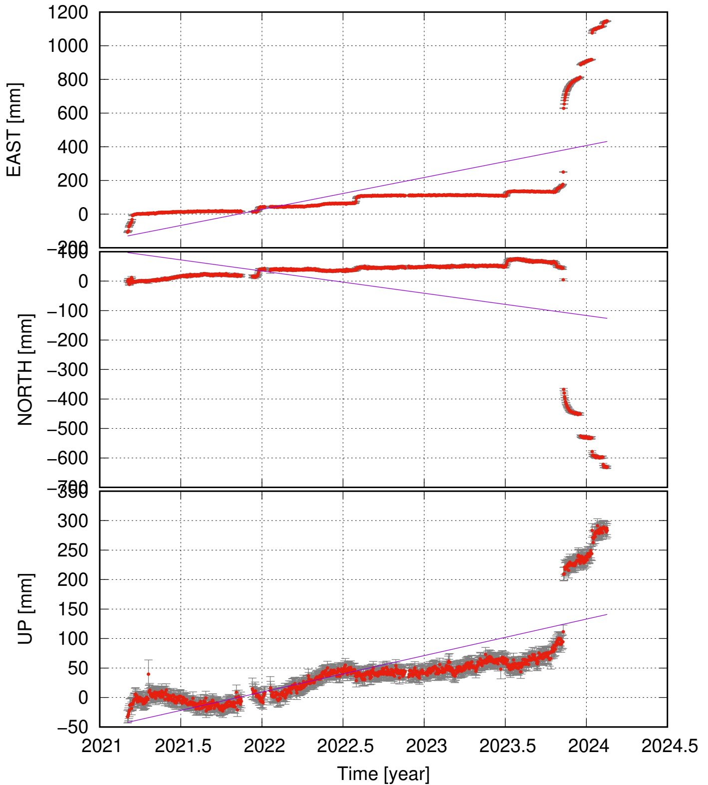
FEFC (63.86, -22.31) time series (ITRF 2014) v_e = 189.78 \pm 67.39 ; v_n = -75.51 \pm 51.45 ; v_u = 61.93 \pm 15.05 mm/yr
