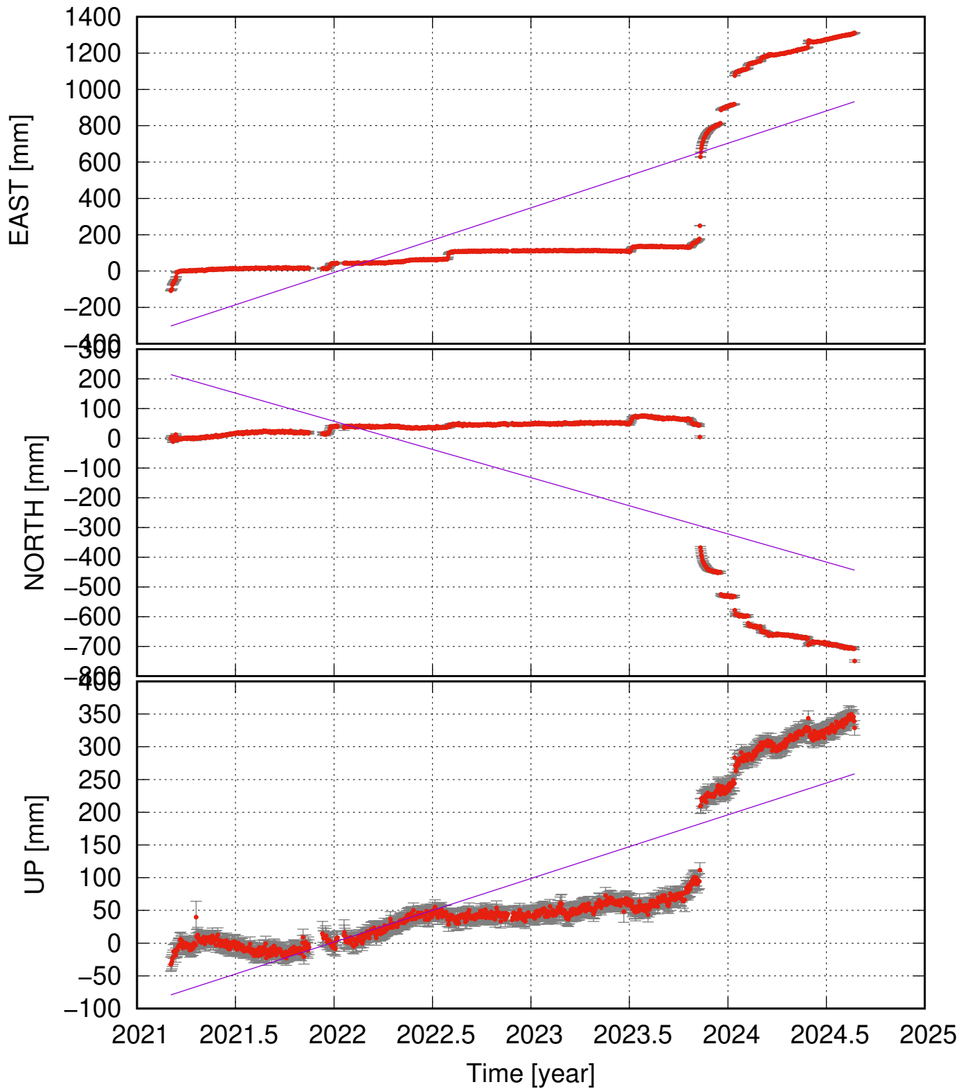
FEFC (63.86, -22.31) time series (ITRF 2014) v_e = 355.72 \pm 81.15 ; v_n = -189.47 \pm 59.03 ; v_u = 97.33 \pm 17.52 mm/yr
