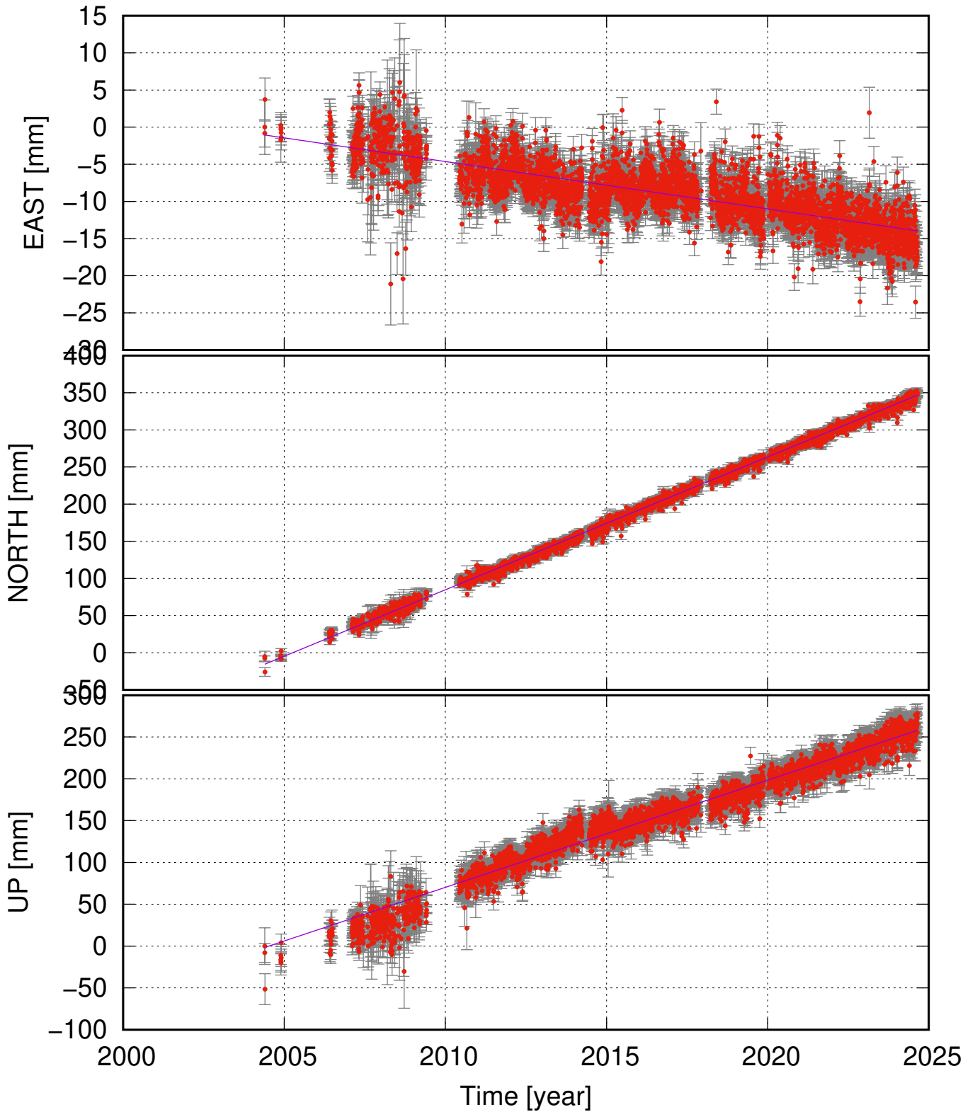
FEDG (64.03, -19.69) time series (ITRF 2014) v_e = -0.64 \pm 0.12 ; v_n = 17.89 \pm 0.20 ; v_u = 12.82 \pm 0.56 mm/yr
