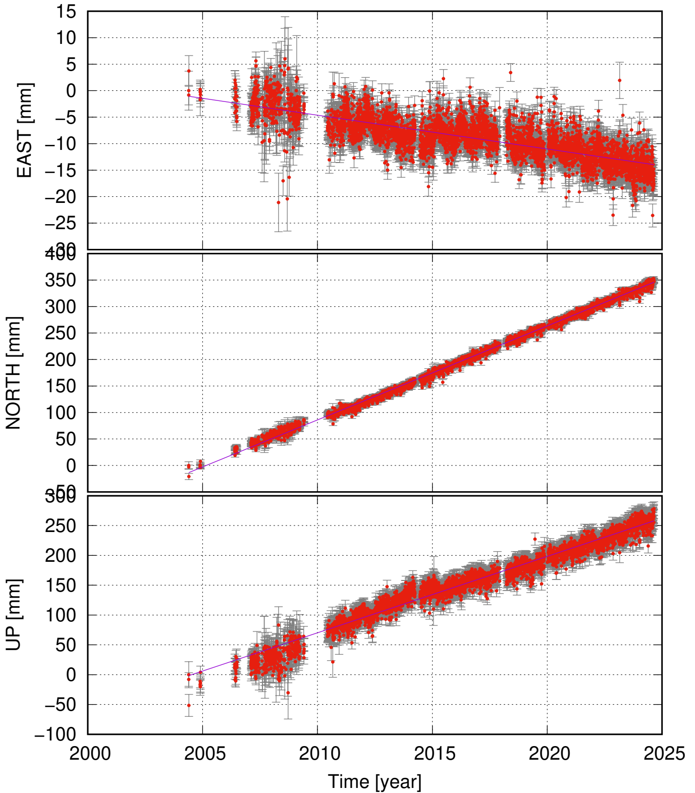
FEDG (64.03, -19.69) time series (ITRF 2014) v_e = -0.64 \pm 0.12 ; v_n = 17.73 \pm 0.22 ; v_u = 12.82 \pm 0.56 mm/yr
