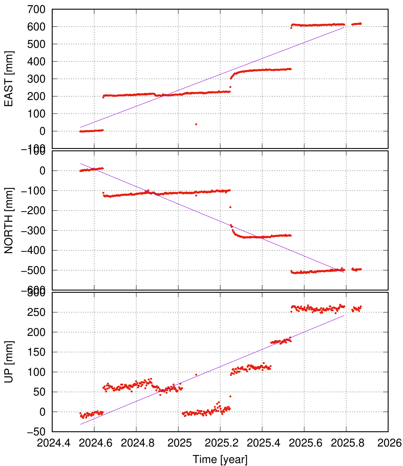
FAGD ( , ) time series (IGb20) ve = +- ; vn = +- ; vu = +- mm/yr
