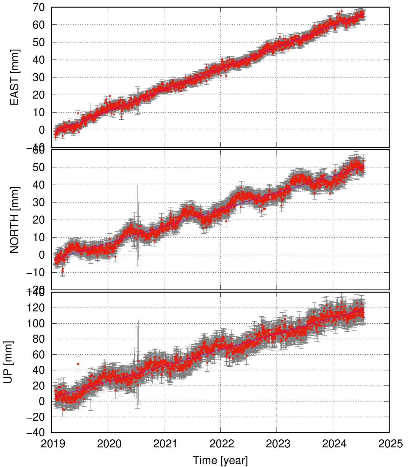
FAGC (63.87, -16.65) time series (ITRF 2014) v_e = 12.19 \pm 0.30 ; v_n = 9.59 \pm 0.51 ; v_u = 20.53 \pm 1.12 mm/yr
