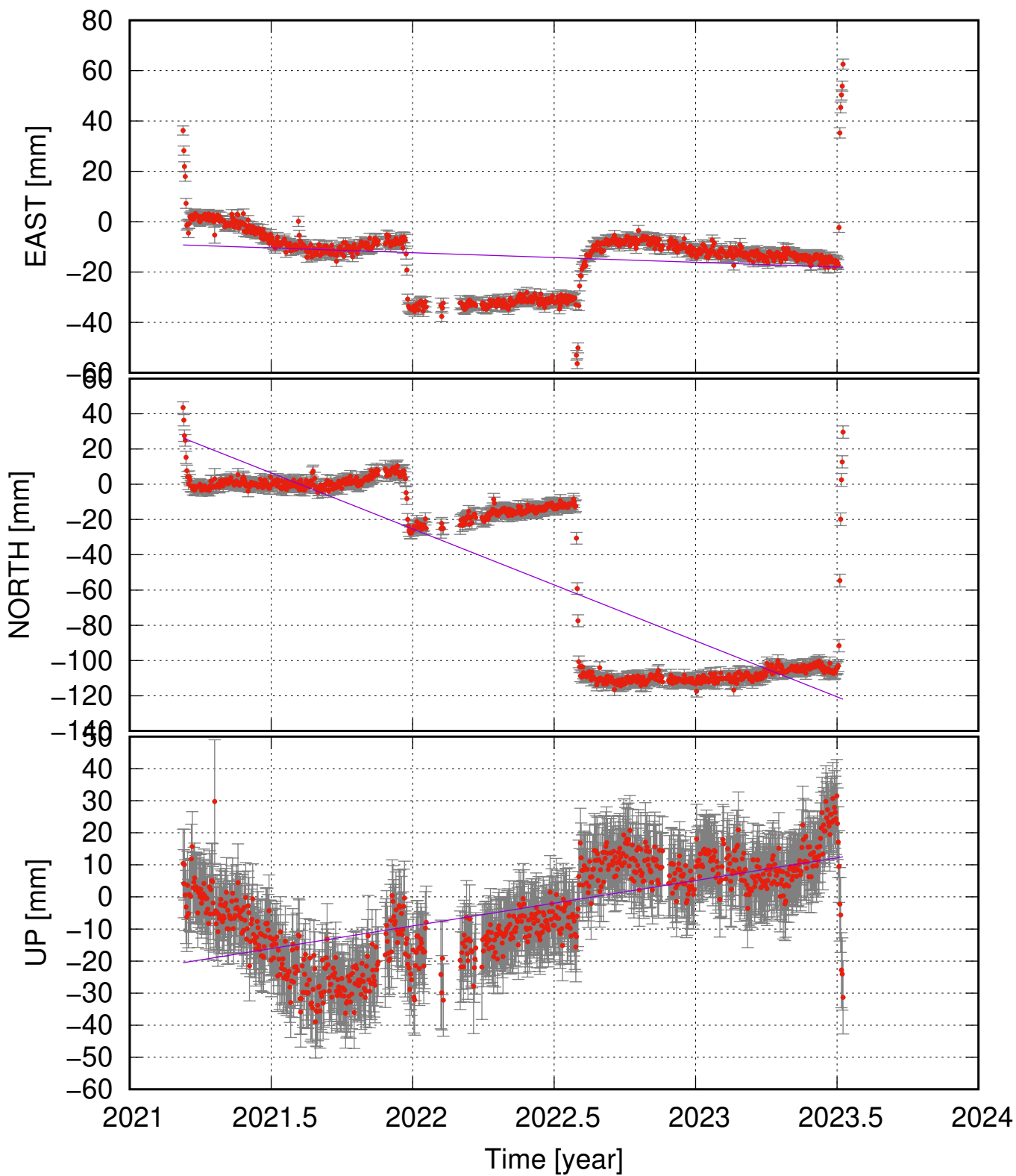
FAFC (63.91, -22.22) time series (ITRF 2014) v_e = -3.78 \pm 5.14 ; v_n = -63.51 \pm 11.24 ; v_u = 14.16 \pm 4.71 mm/yr
