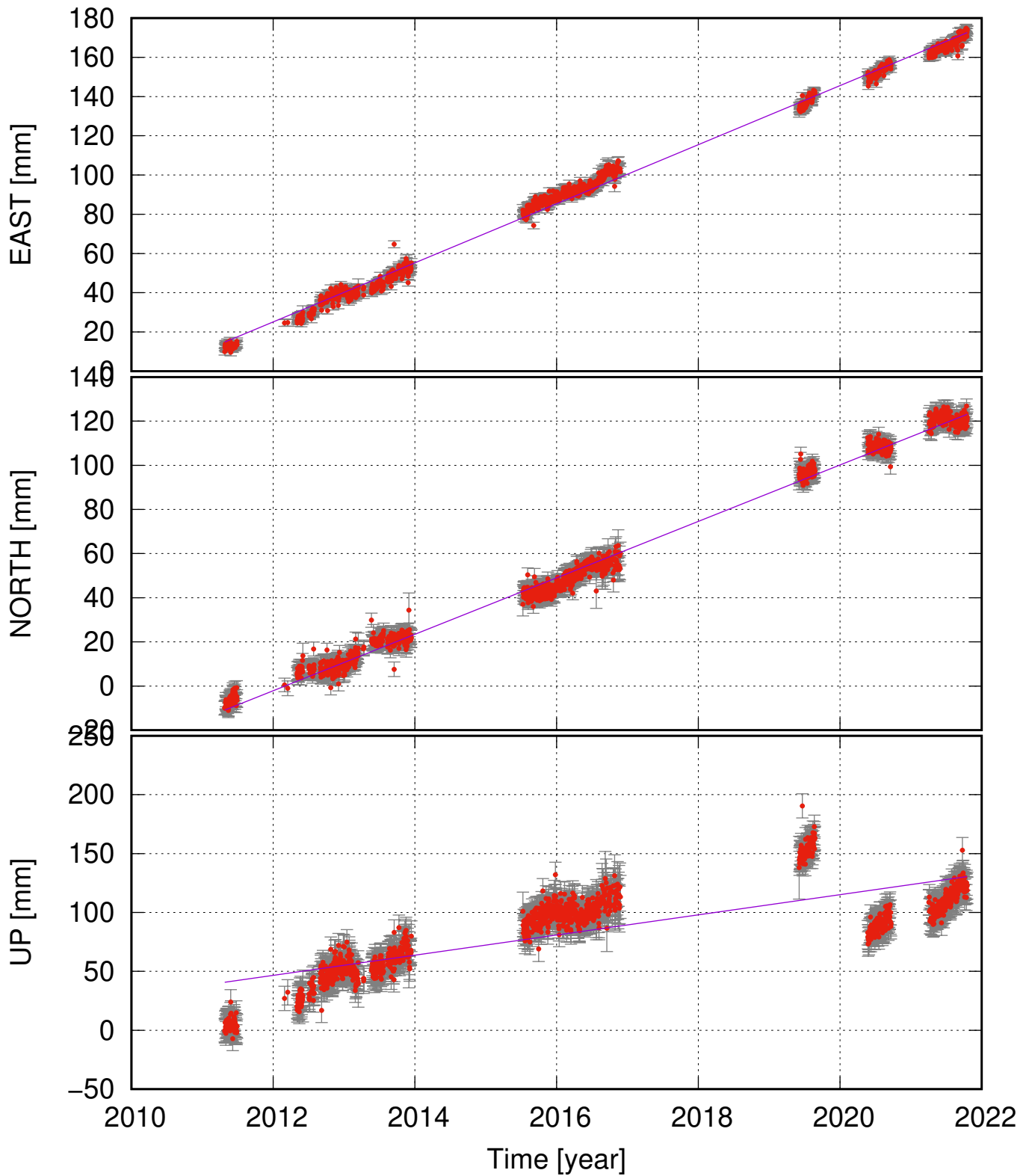
EYVI (64.23, -15.80) time series (ITRF 2014) v_e = 15.06 \pm 0.30 ; v_n = 12.78 \pm 0.32 ; v_u = 8.57 \pm 2.11 mm/yr
