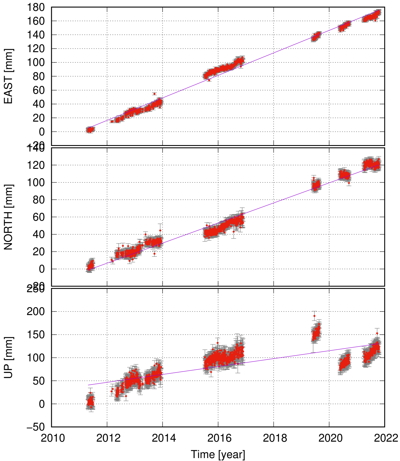
EYVI (64.23, -15.80) time series (ITRF 2014) v_e = 16.25 \pm 0.53 ; v_n = 11.60 \pm 0.52 ; v_u = 8.57 \pm 2.11 mm/yr
