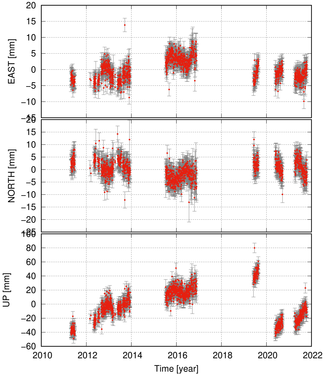
EYVI residual time series (some major events removed as well)
