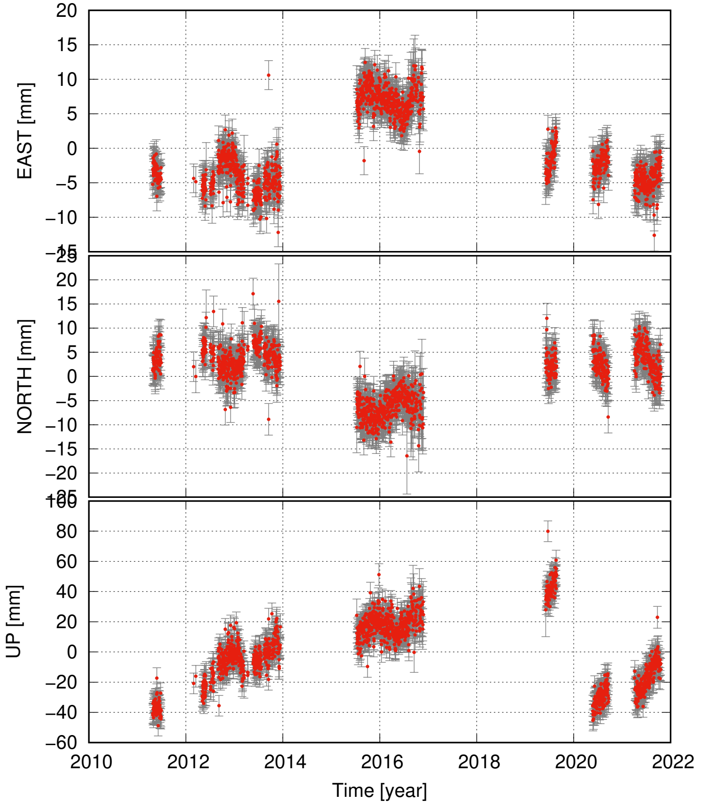
EYVI residual time series
