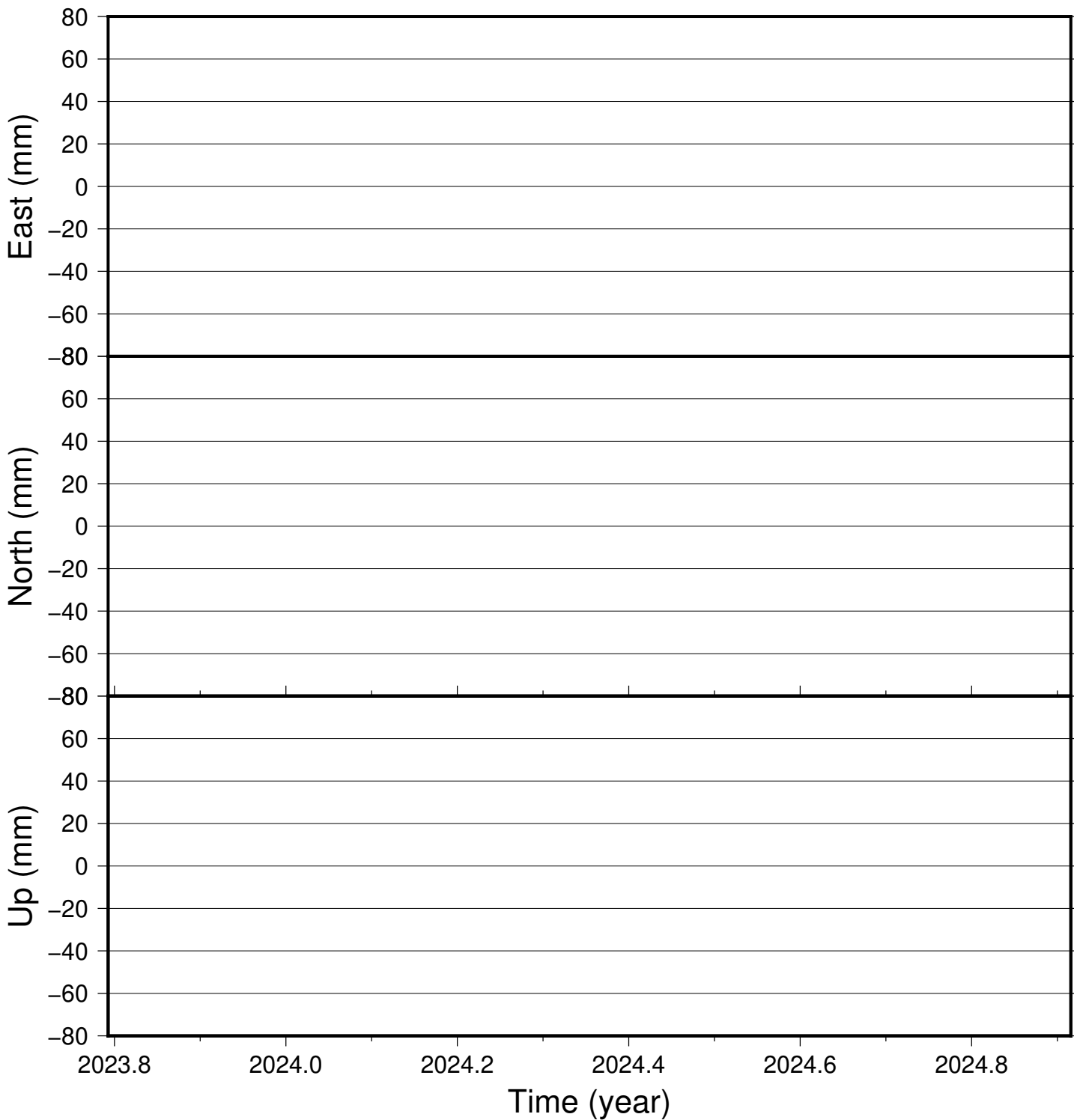
EYVI time series (IGS 2014), last 400 days
