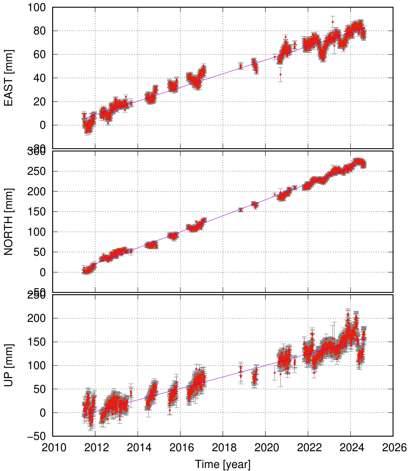
ENTC (63.70, -19.18) time series (ITRF 2014) v_e = 5.81 \pm 0.33 ; v_n = 19.86 \pm 0.45 ; v_u = 12.18 \pm 1.09 mm/yr
