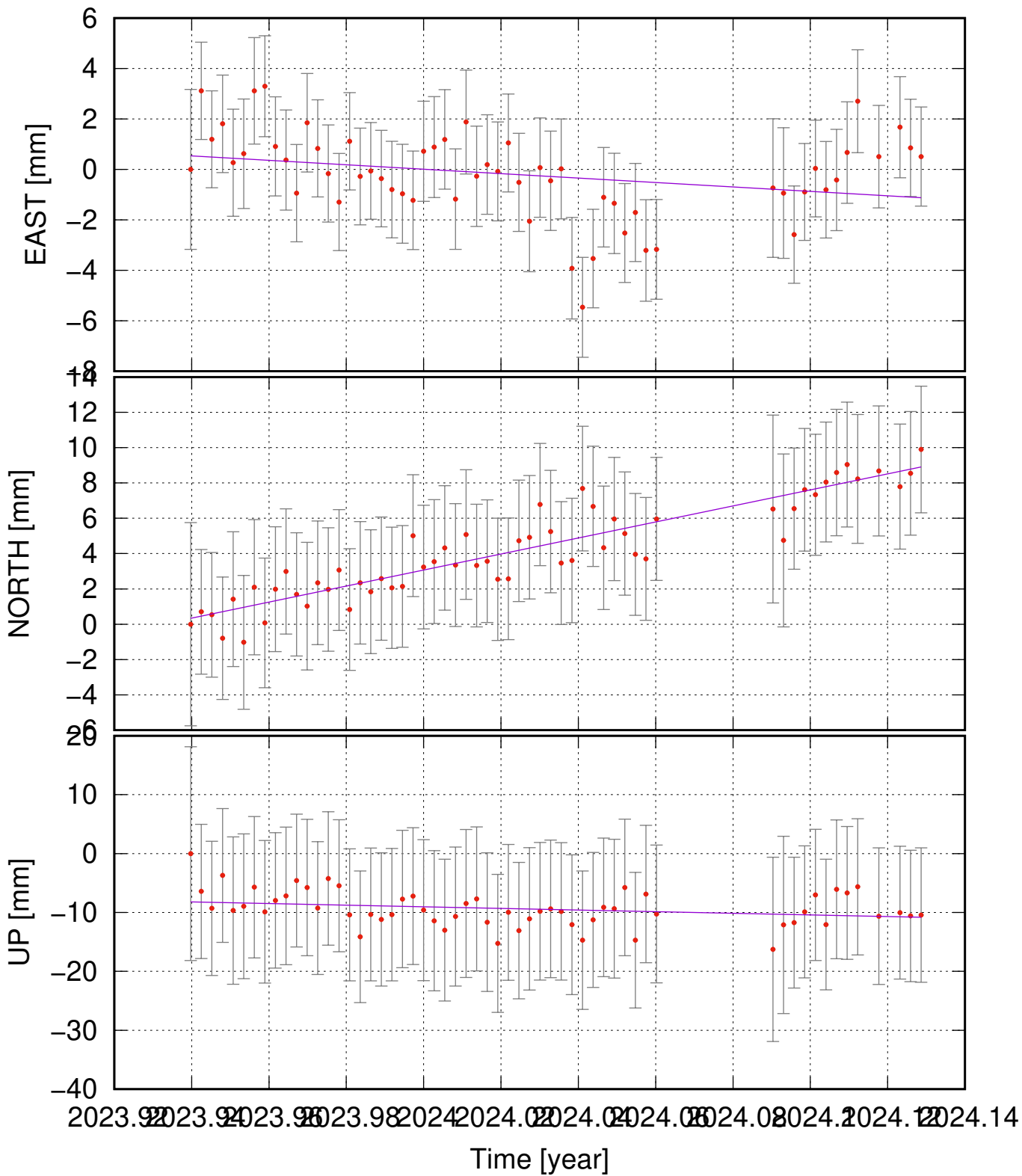
ELEY (63.74, -22.96) time series (ITRF 2014) ve = -8.78 \pm 8.88 ; vn = 45.35 \pm 5.81 ; vu = -13.74 \pm 15.67 mm/yr
