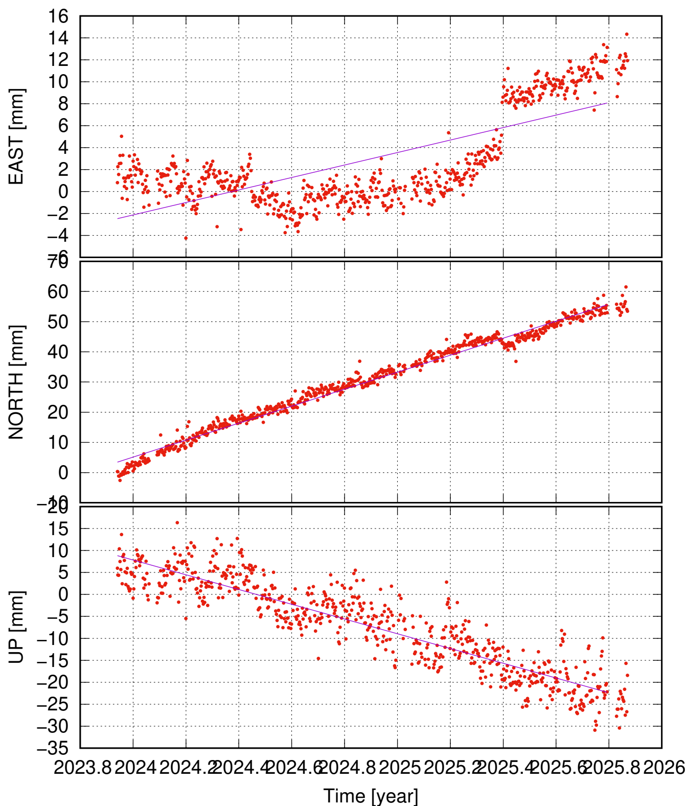
ELEY ( , ) time series (IGb20) ve = +- ; vn = +- ; vu = +- mm/yr
