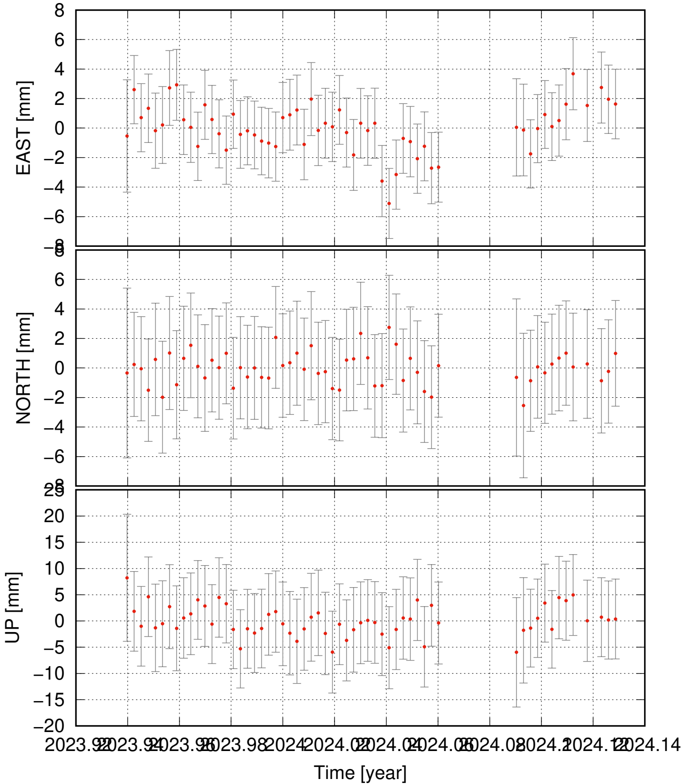
ELEY residual time series (some major events removed as well)
