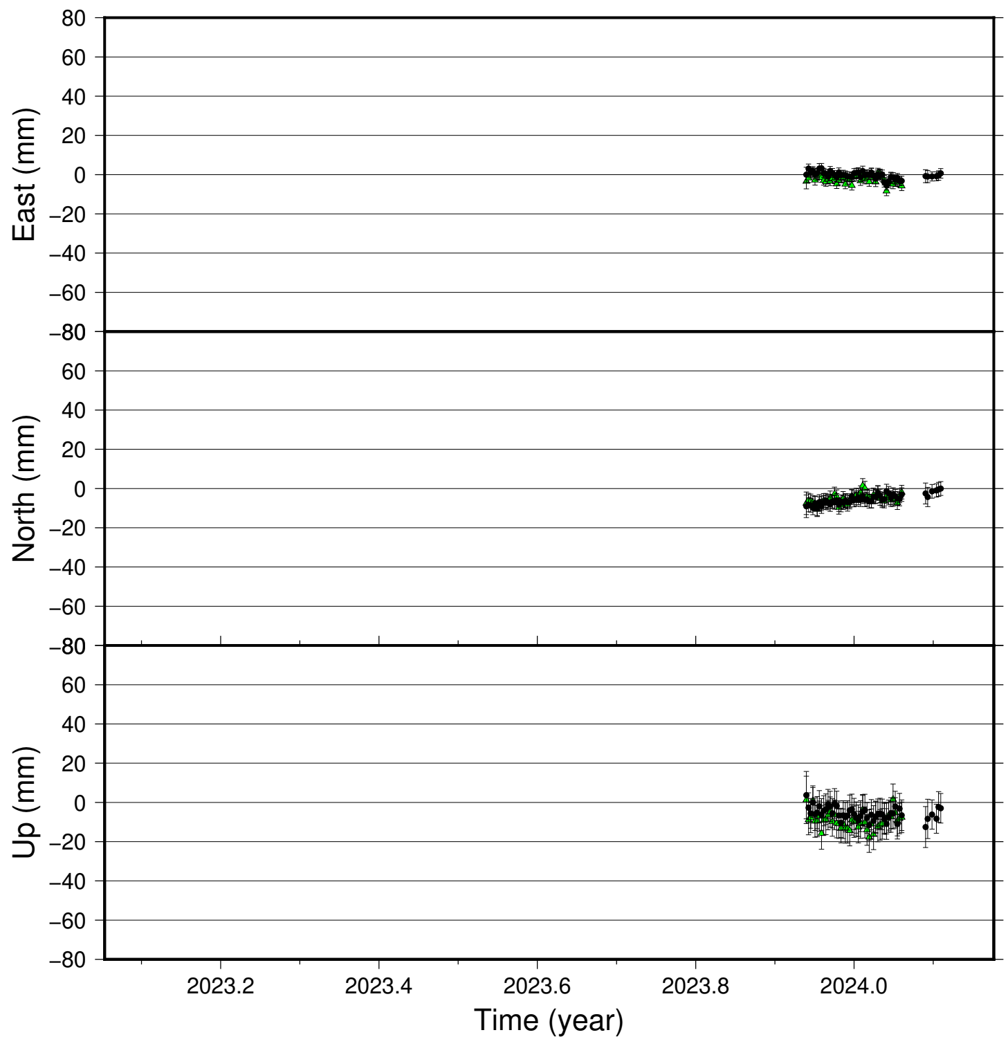
ELEY time series (IGS 2014), last 400 days
