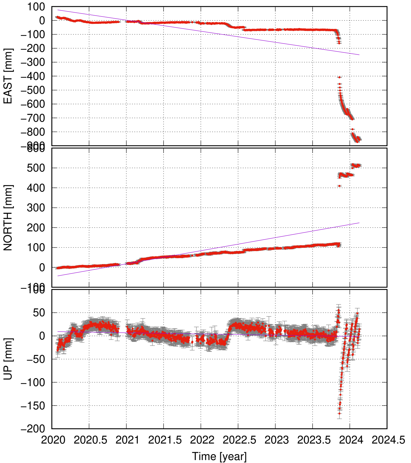
ELDC (63.86, -22.53) time series (ITRF 2014) v_e = -79.58 \pm 37.29 ; v_n = 65.96 \pm 20.55 ; v_u = -2.63 \pm 4.65 mm/yr
