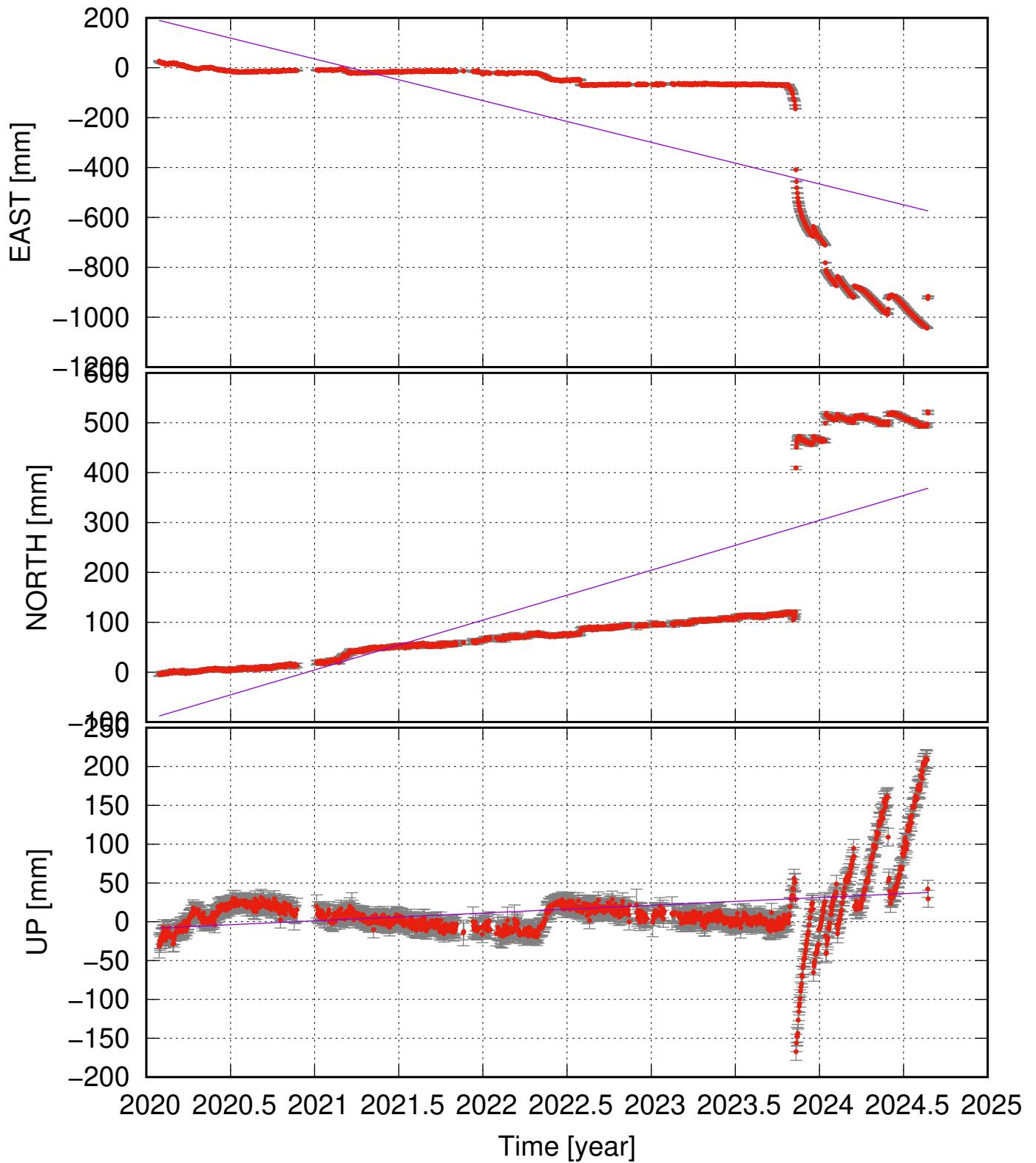
ELDC (63.86, -22.53) time series (ITRF 2014) v_e = -167.09 \pm 50.97 ; v_n = 99.92 \pm 23.32 ; v_u = 10.04 \pm 8.08 mm/yr
