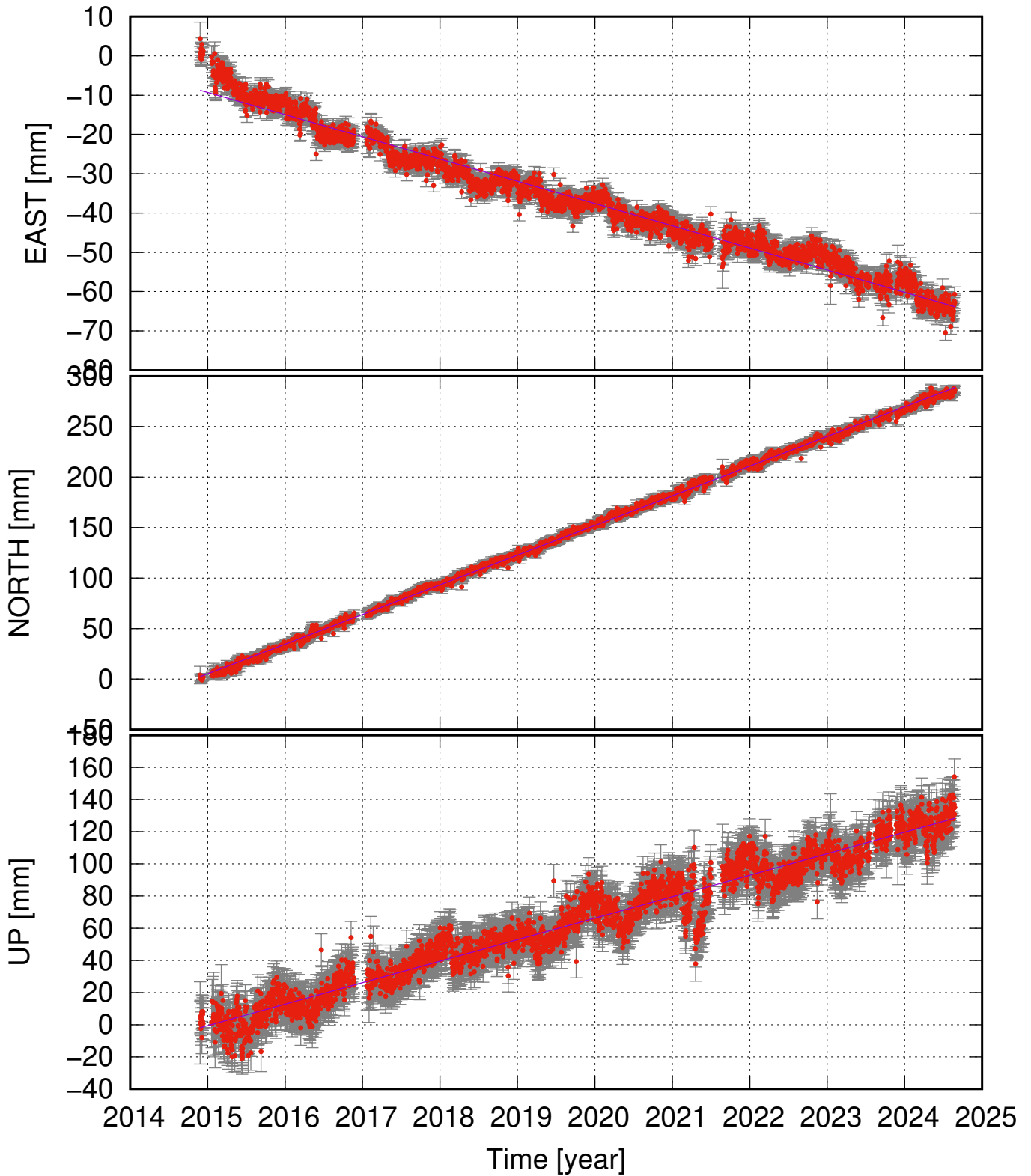
DYNY (65.02, -17.12) time series (ITRF 2014) v_e = -5.65 \pm 0.27 ; v_n = 29.36 \pm 0.27 ; v_u = 13.37 \pm 0.87 mm/yr
