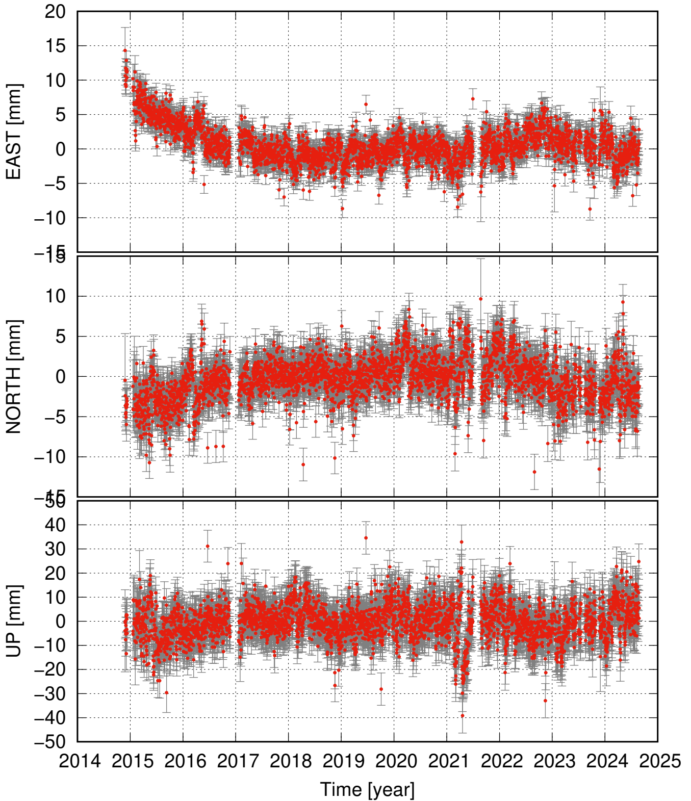
DYNY detrended and seasonal signal removed
