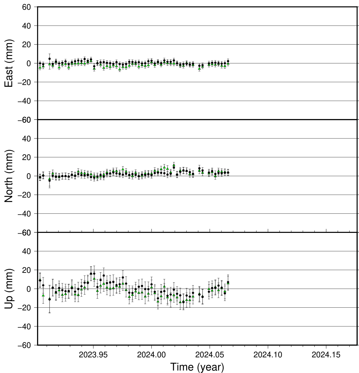
DYNY time series (IGS 2014), last 100 days
