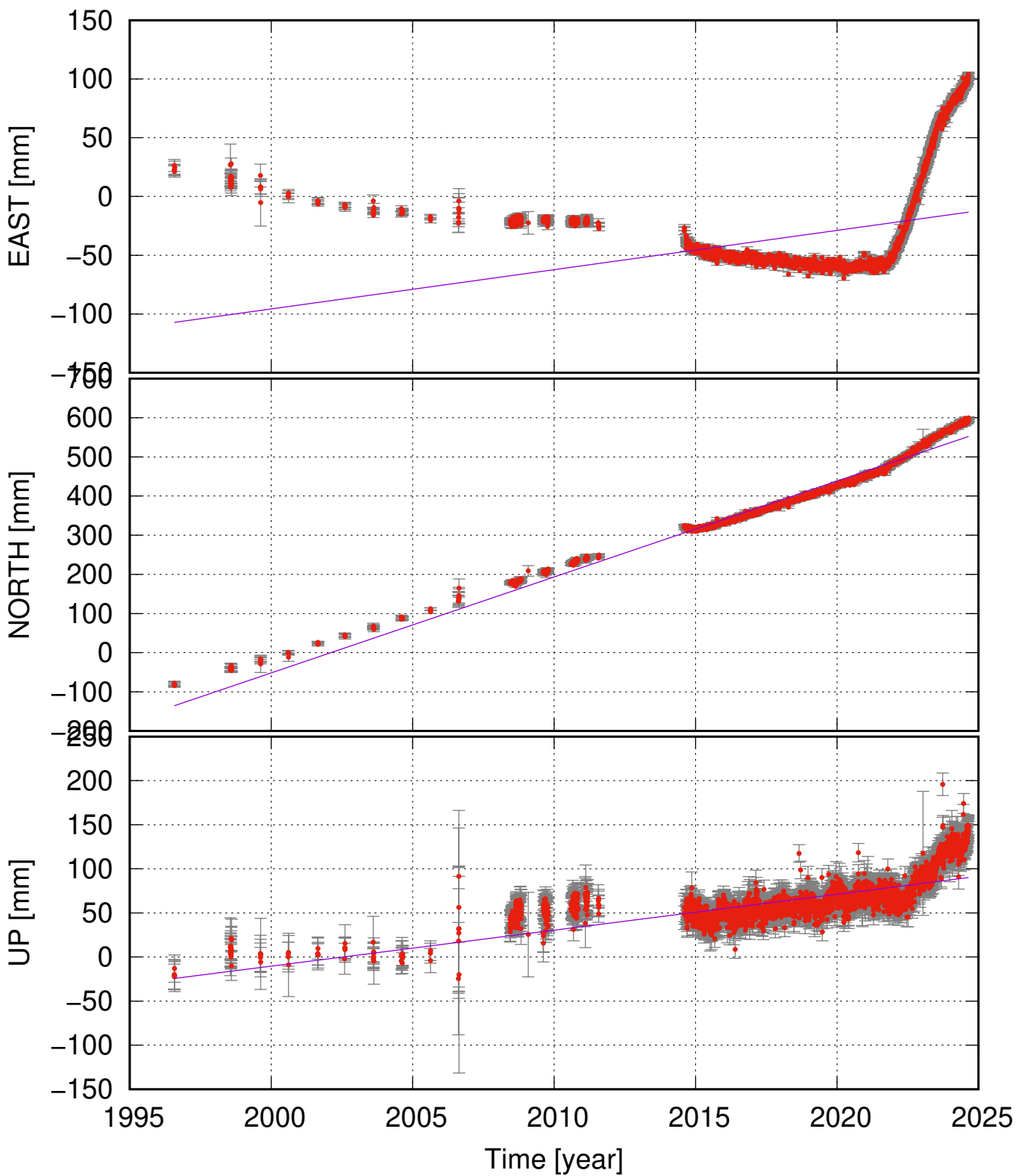
DYNG (65.06, -16.65) time series (ITRF 2014) v_e = 3.34 \pm 1.49 ; v_n = 24.50 \pm 0.61 ; v_u = 4.08 \pm 0.62 mm/yr
