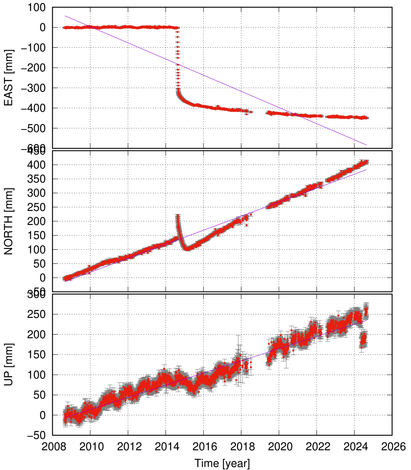
DYNC (64.79, -17.37) time series (ITRF 2014) v_e = -40.06 \pm 6.41 ; v_n = 24.83 \pm 1.17 ; v_u = 15.09 \pm 0.93 mm/yr
