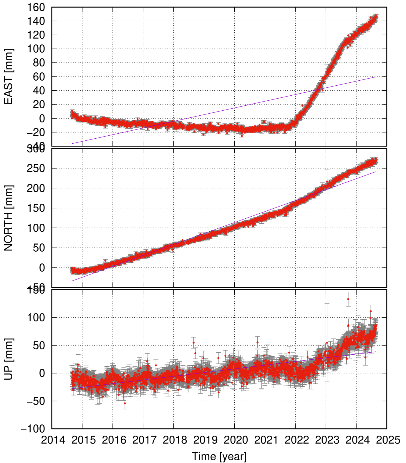
DYNA (65.06, -16.65) time series (ITRF 2014) v_e = 9.62 \pm 3.44 ; v_n = 27.58 \pm 1.26 ; v_u = 6.65 \pm 1.45 mm/yr
