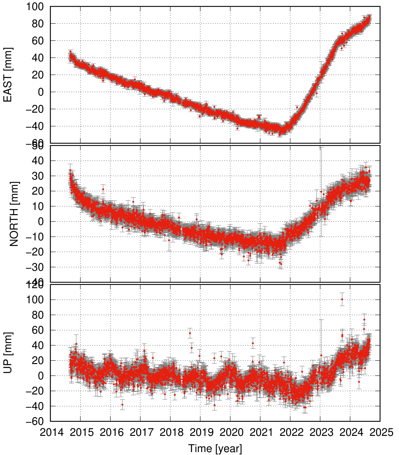
DYNA residual time series (some major events removed as well)
