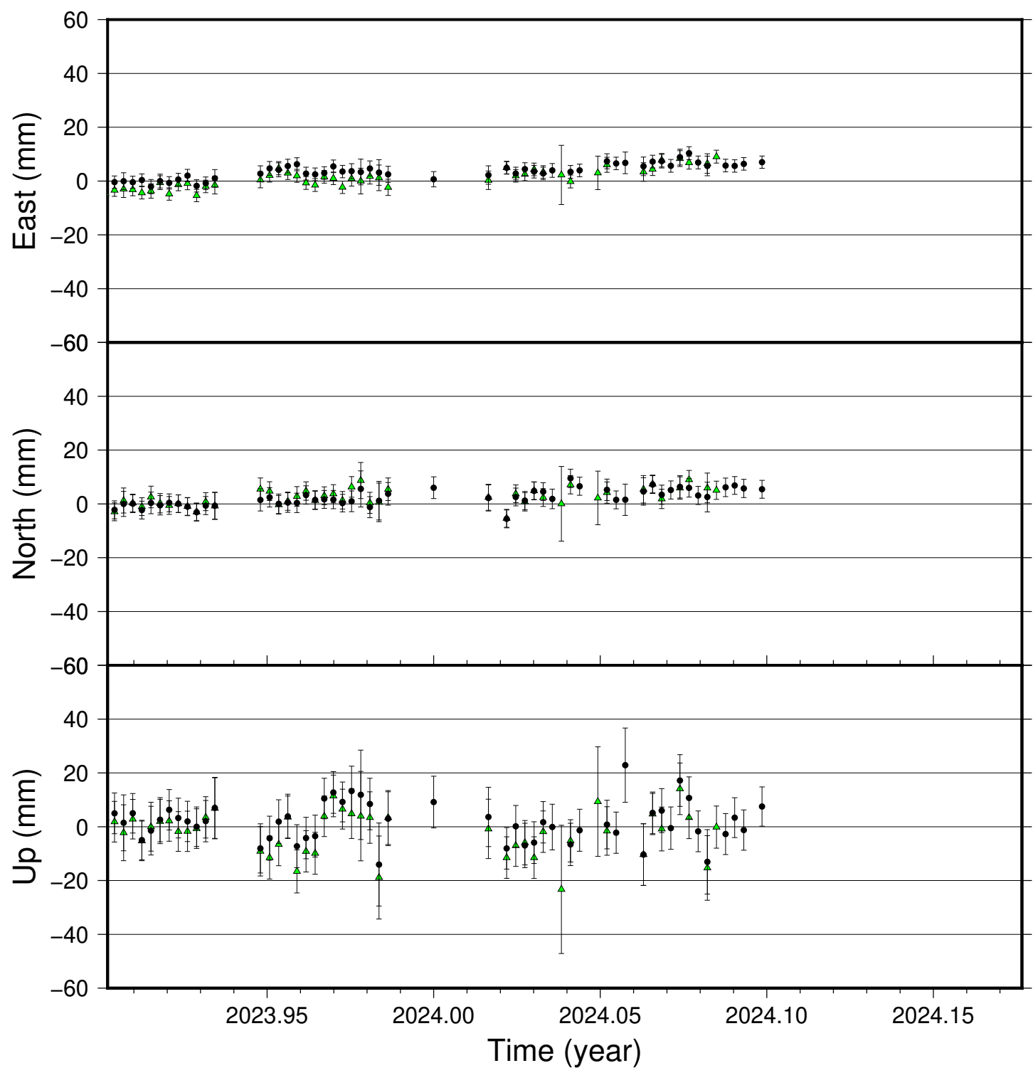
DYNA time series (IGS 2014), last 100 days
