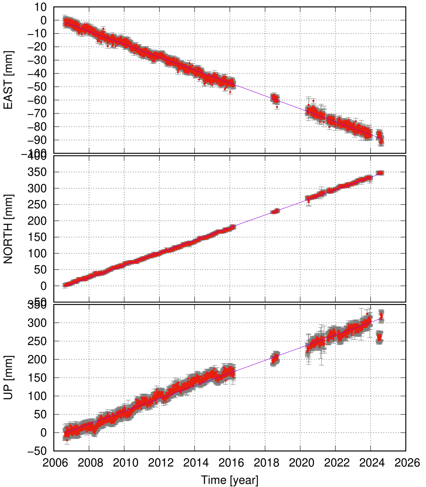
BUDH (64.24, -19.32) time series (ITRF 2014) v_e = -4.86 \pm 0.09 ; v_n = 19.29 \pm 0.18 ; v_u = 17.38 \pm 0.57 mm/yr
