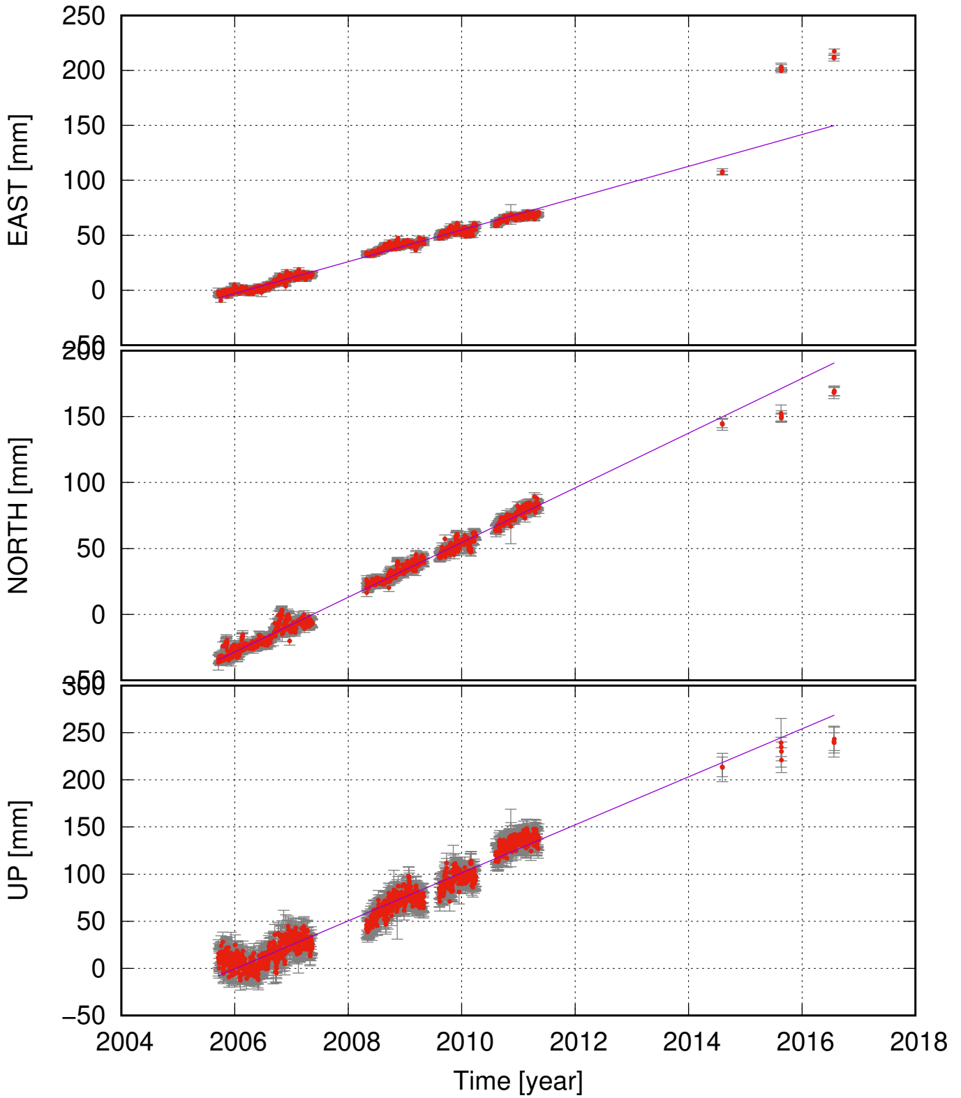
BRUJ (64.83, -16.09) time series (ITRF 2014) v_e = 14.45 \pm 0.49 ; v_n = 20.73 \pm 0.32 ; v_u = 25.47 \pm 0.85 mm/yr
