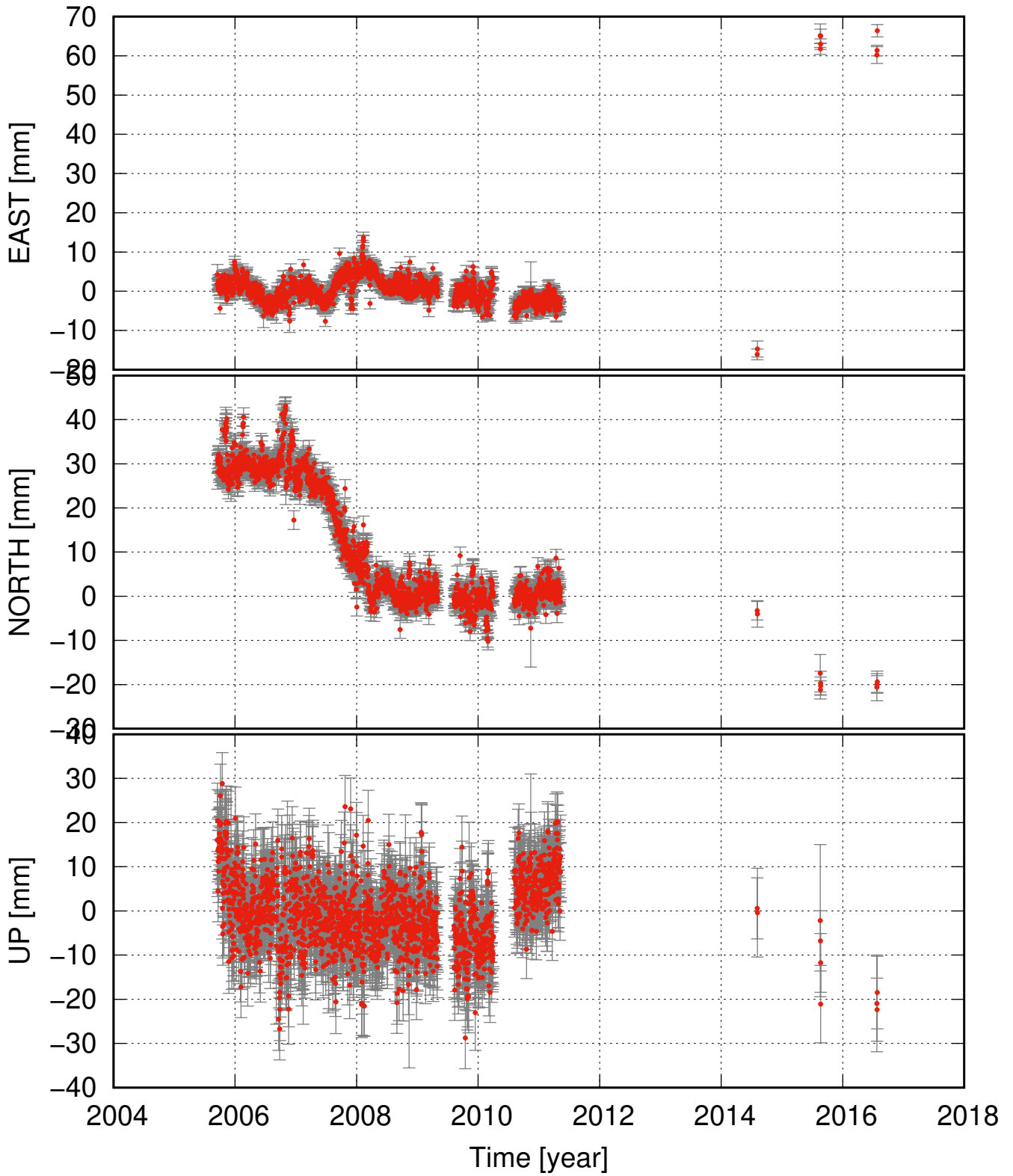
BRUJ detrended and seasonal signal removed
