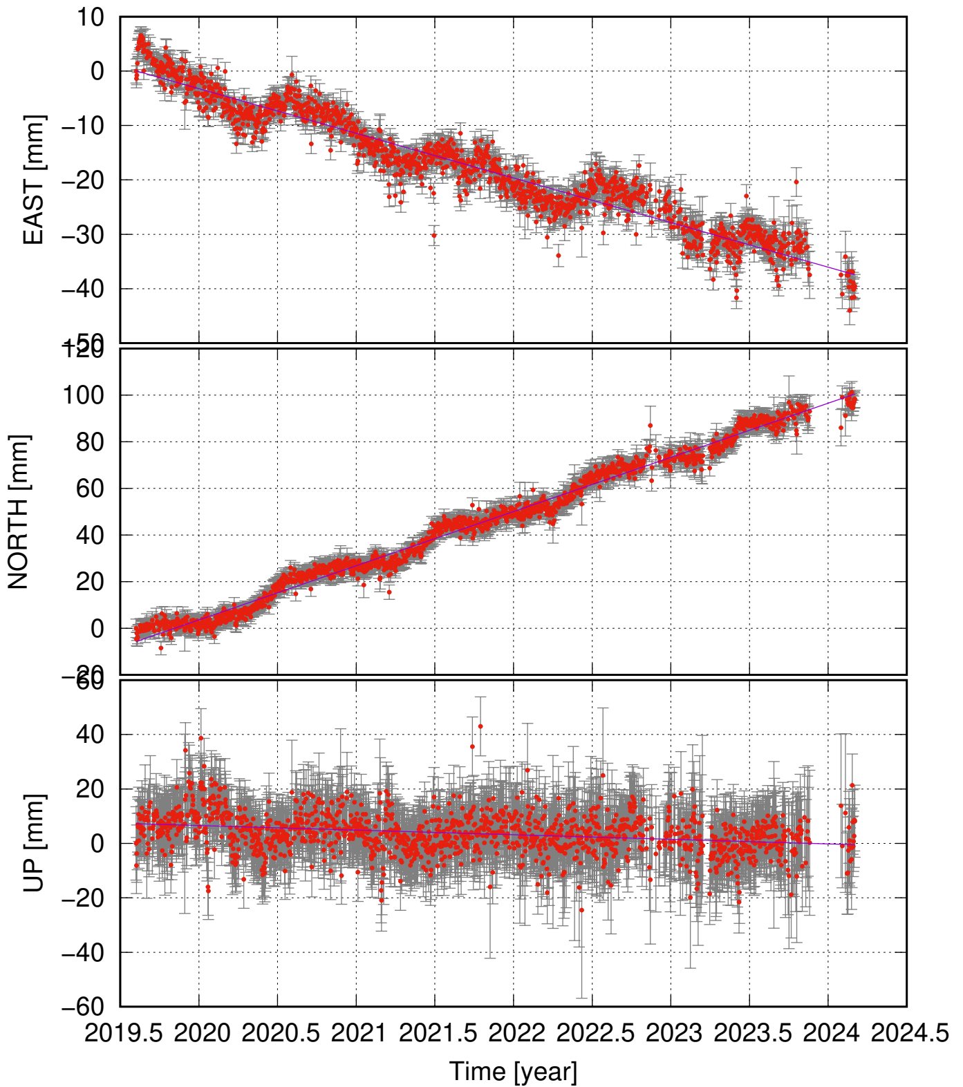
BRTT (66.12, -17.91) time series (ITRF 2014) v_e = -8.20 \pm 0.64 ; v_n = 23.24 \pm 0.74 ; v_u = -1.68 \pm 1.53 mm/yr
