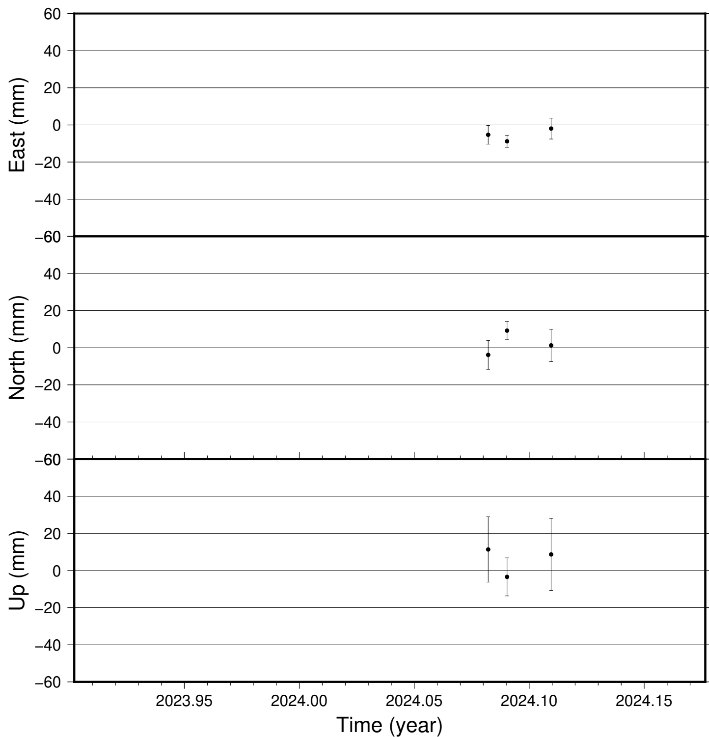
BRTT time series (IGS 2014), last 100 days
