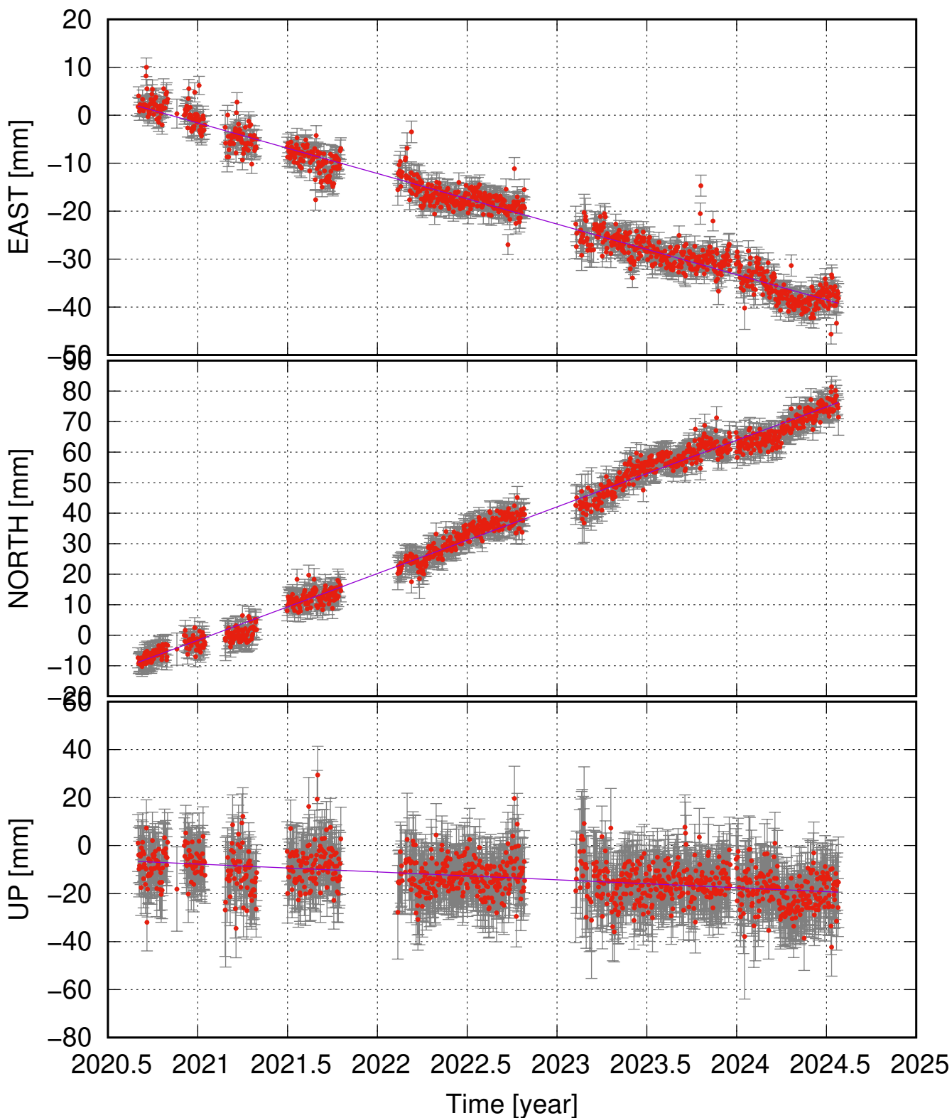
BRİK (66.12, -18.61) time series (ITRF 2014) v_e = -10.54 \pm 0.60 ; v_n = 21.85 \pm 0.72 ; v_u = -3.28 \pm 1.91 mm/yr
