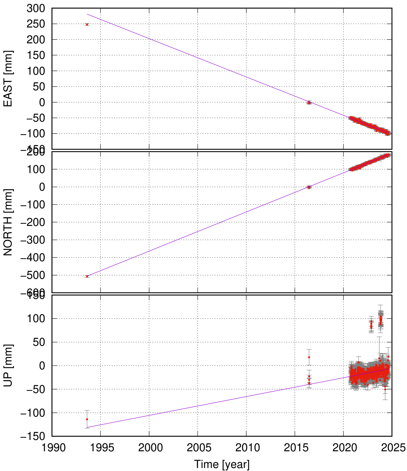
BLON (65.40, 65.40) time series (ITRF 2014) v_e = -12.23 \pm 0.06 ; v_n = 22.18 \pm 0.07 ; v_u = 4.00 \pm 0.58 mm/yr
