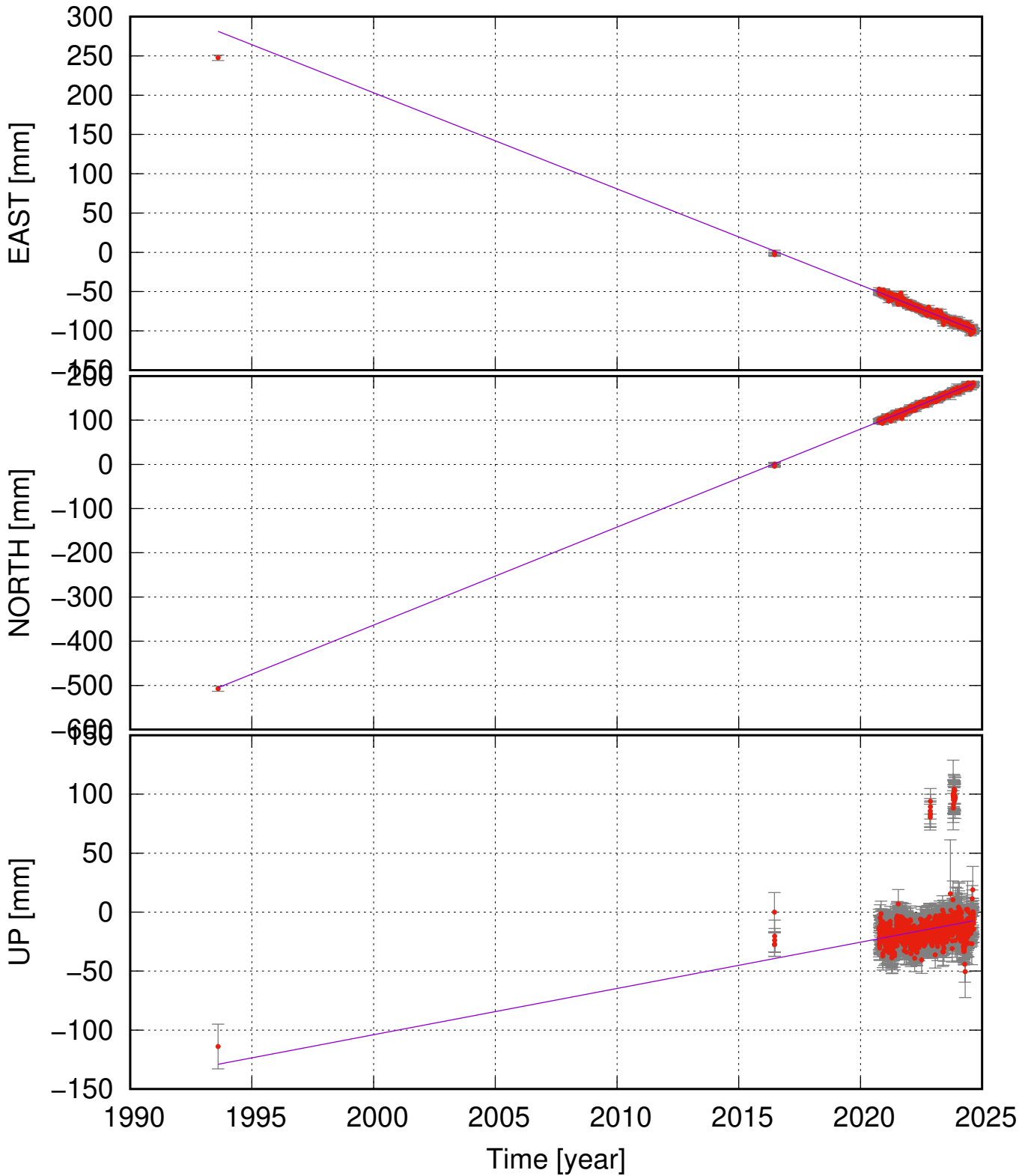
BLON (65.40, 65.40) time series (ITRF 2014) v_e = -12.24 \pm 0.06 ; v_n = 22.17 \pm 0.07 ; v_u = 3.92 \pm 0.58 mm/yr
