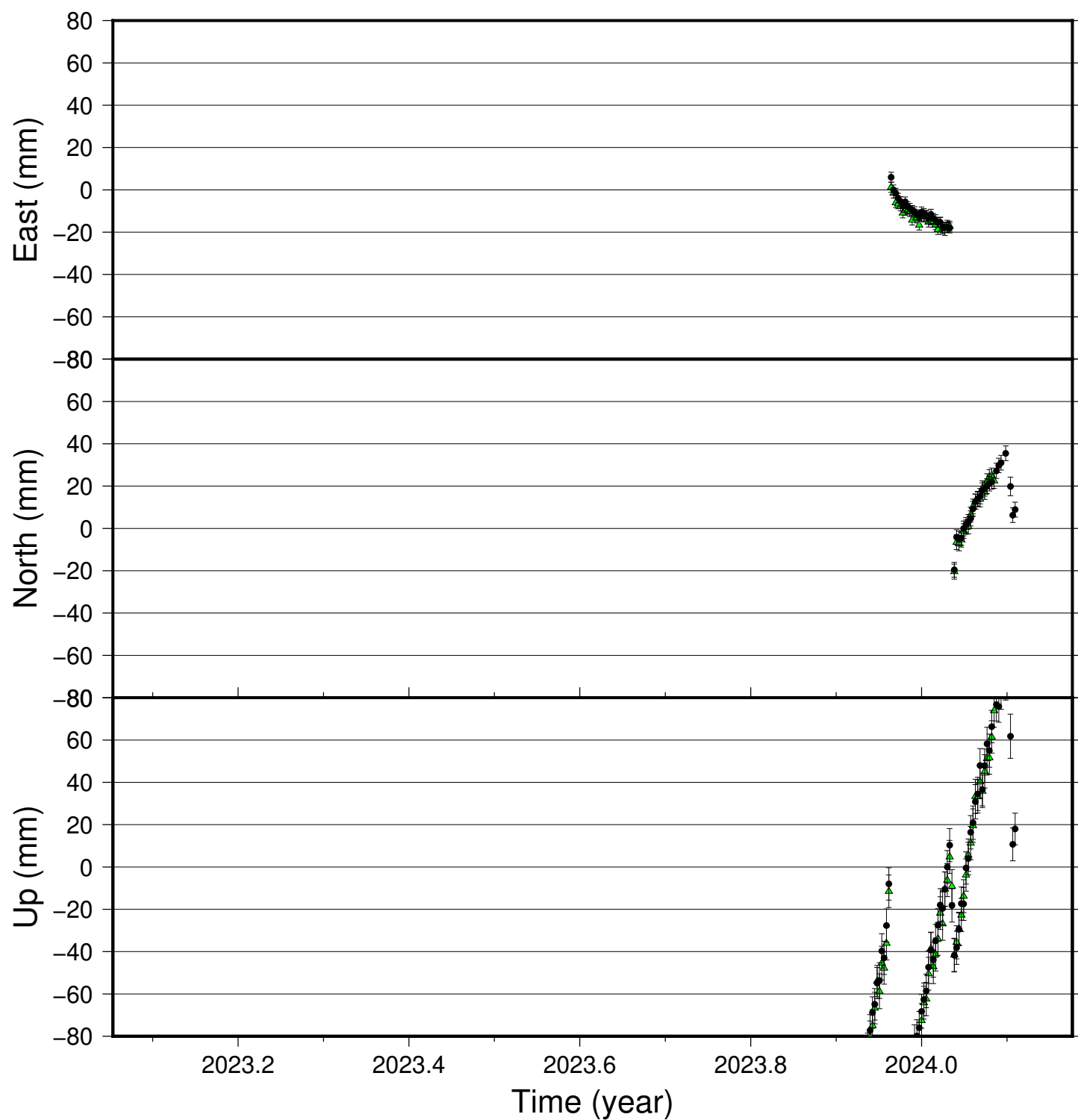
BLAL time series (IGS 2014), last 400 days
