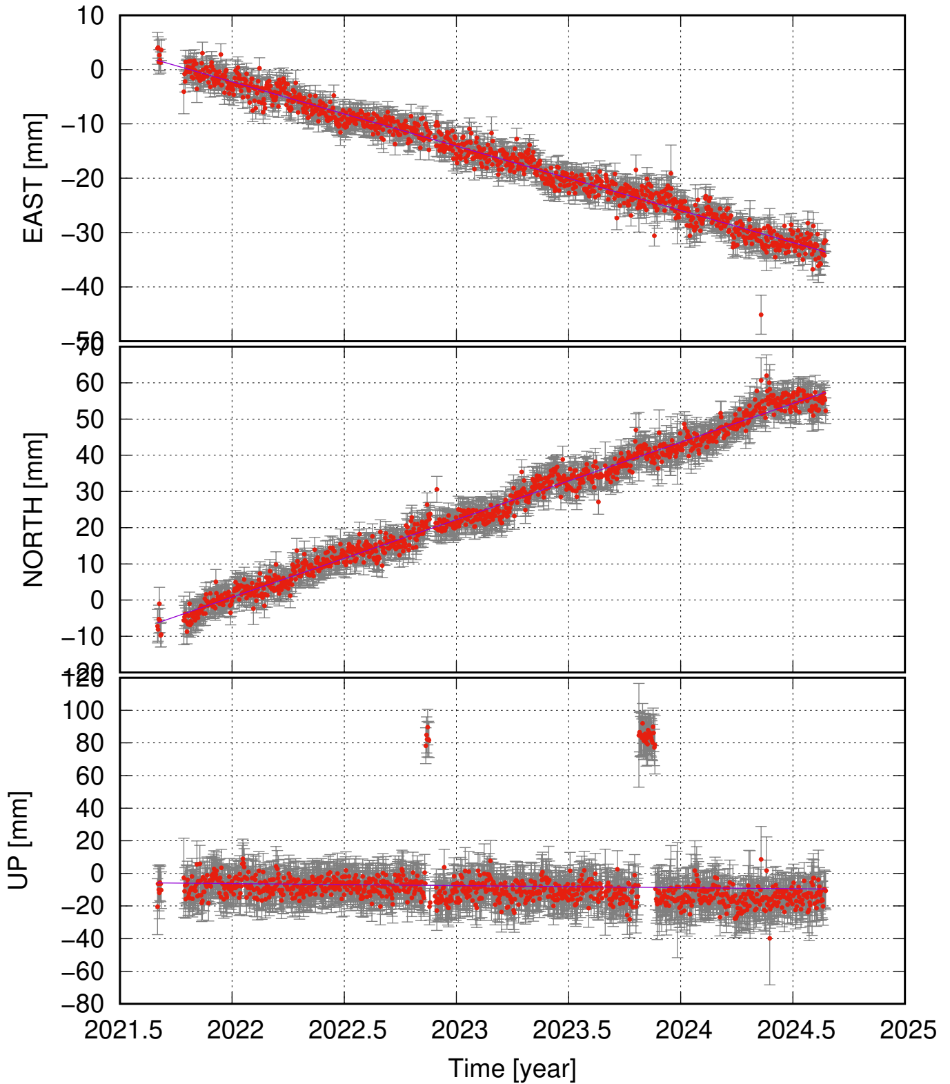
BJTV (65.50, -24.53) time series (ITRF 2014) v_e = -11.84 \pm 0.54 ; v_n = 21.36 \pm 0.74 ; v_u = -1.27 \pm 5.92 mm/yr
