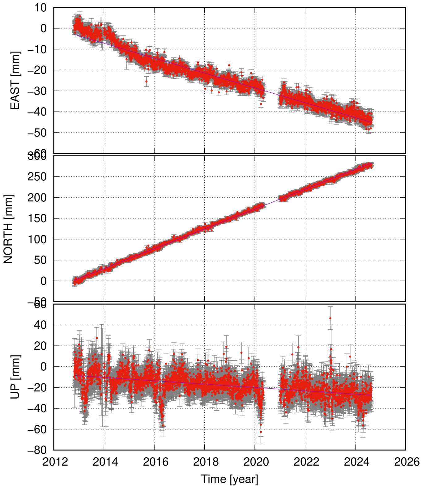
BJAC (65.61, -16.83) time series (ITRF 2014) v_e = -3.56 \pm 0.21 ; v_n = 23.73 \pm 0.25 ; v_u = -1.60 \pm 0.74 mm/yr
