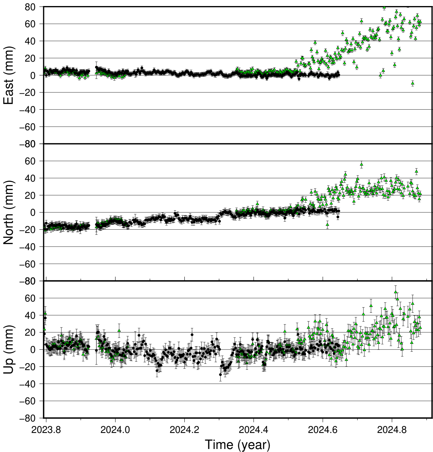
BJAC time series (IGS 2014), last 400 days
