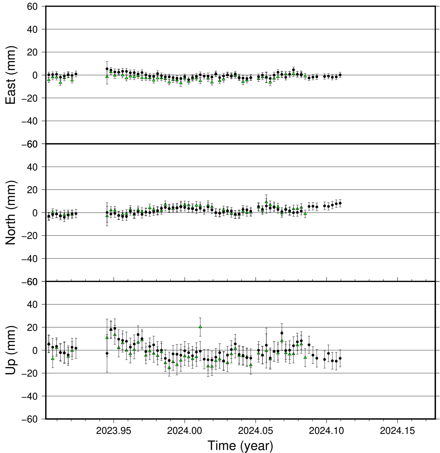
BJAC time series (IGS 2014), last 100 days
