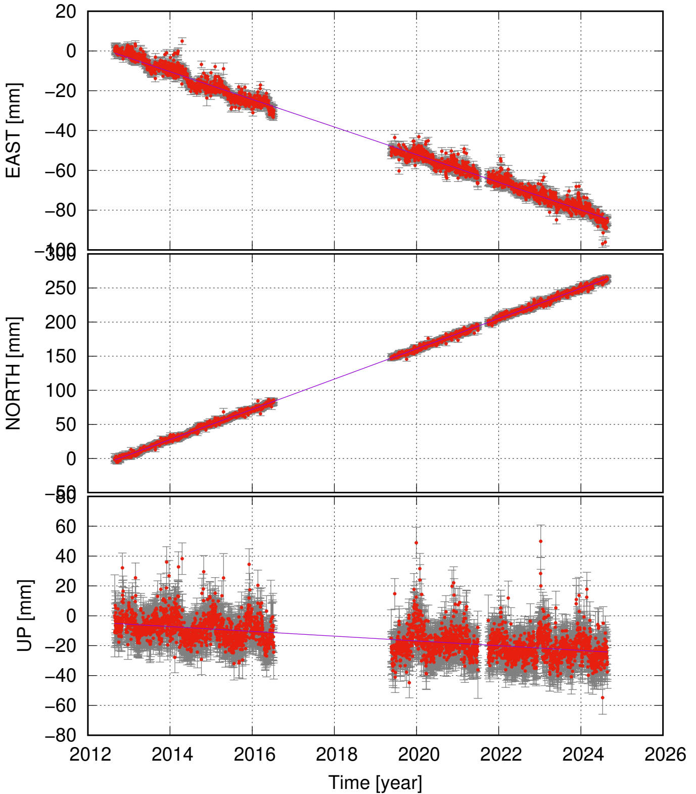
BAUG (66.04, -17.33) time series (ITRF 2014) v_e = -6.95 \pm 0.20 ; v_n = 22.18 \pm 0.17 ; v_u = -1.60 \pm 0.70 mm/yr
