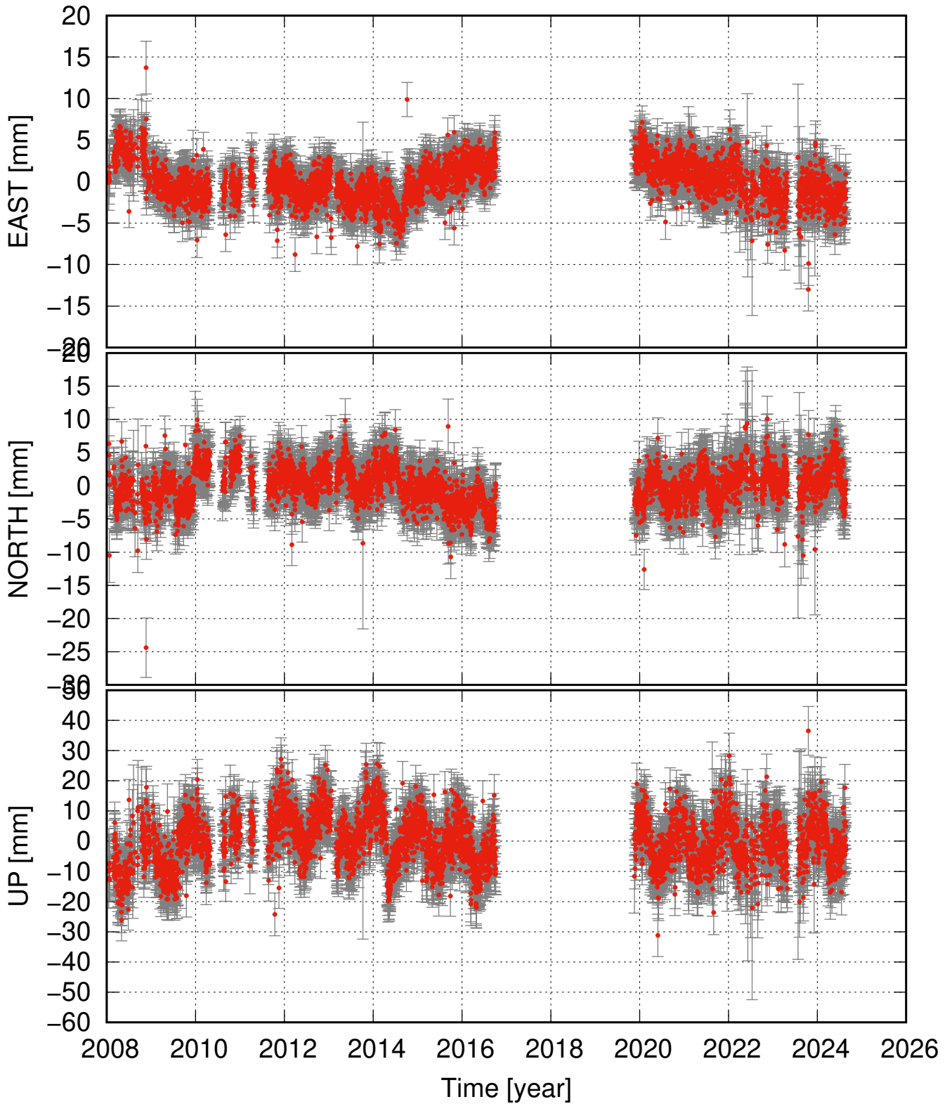
BALD residual time series (some major events removed as well)
