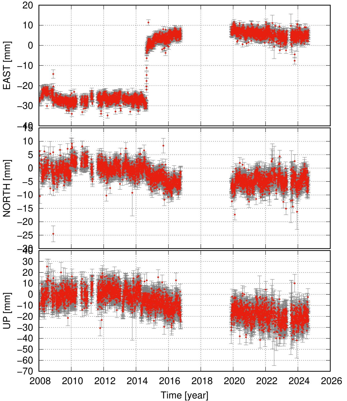
BALD detrended and seasonal signal removed
